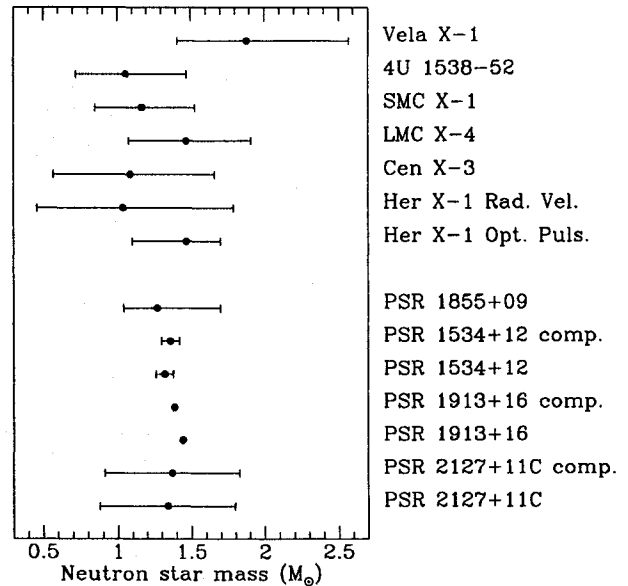
Fig. 1. The currently known masses of neutron stars. Shown are both the masses for the X-ray pulsars (Table 3) and for the radio pulsars (and their companions; Table 1). The error bars indicate 95% confidence limits. For the radio pulsars, these have been obtained by multiplying the 1\sigma errors listed in Table 1 by two (except for PSR 1855+09, for which we read M_{\text{pulsar}} = 1.27^{+0.43}_{-0.23} from Fig. 8 of Ryba & Taylor 1991)
