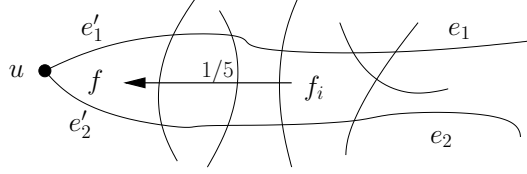
Figure 1: The first round of charges redistribution
