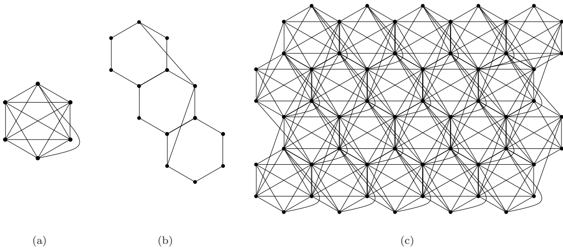
Figure 3: A construction for a quasi-planar graph with n vertices and 7n - O(1) edges.
