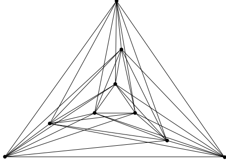
Figure 2: K_9 drawn as a quasi-planar geometric graph.
