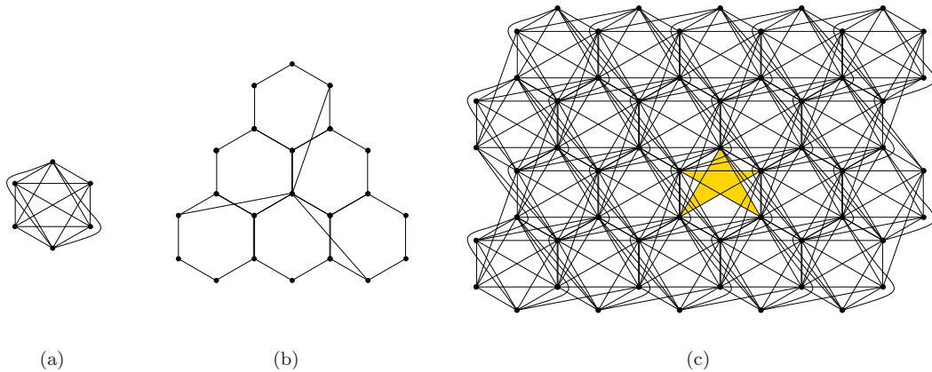
Figure 4: A generalized topological graph satisfying the conditions of Theorem 3.
