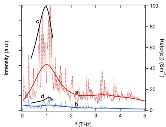
FIG. 4. (Color online) The Fourier transform of the autocorrelation function \langle V(0)V(t) \rangle for both the coupling between the HOMO levels (a, in red) and LUMO levels (b, in blue). For simplicity, we show an average of the spectral density obtained for all the inequivalent pairs of nearest neighbors in the a-b plane since the difference between them is negligible when the broadening is introduced. The dotted traces show the original curves, whereas the solid ones represent the case of adding a broadening of 0.3 THz to the original spectra. The black traces c and d show the conductivity (depicted on the right axis) at t=1.3 ps for 20 K when optically exciting at 400 nm ( c ) and at room temperature when optically exciting at 266 nm ( d ).
