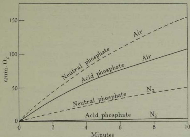
FIG. 1—Effect of pure N_2 on the decomposition of H_2O_2 by a purified catalase preparation: Catalase D (diluted to approximately 10^{-9} M with respect to haematin); 0.3 c.c. 0.3% H_2O_2 ; 0.03M phosphate buffer; T = 19^\circ C .
