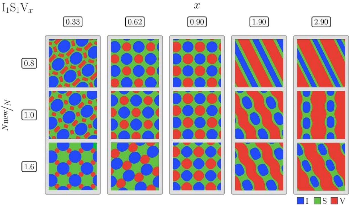
Figure 7. SCFT studies on the effects of simultaneously changing the three Flory-Huggins chi parameters via the ratio N_{new}/N . for the five different samples of ISV- x . ISV-0.33 transformed from [12.6.4] tiling to [8.8.4] tiling and ISV-0.62 changed from [8.8.4] tiling to [6.6.6] tiling as N_{new}/N was increased from 0.8/1 to 1.6. ISV-0.90 retained its [8.8.4] tiling structure for all the N_{new}/N values. ISV-1.9 and ISV-2.9 transformed from CYLULAM structure to LAM-3 structure as N_{new}/N was reduced from 1/1.6 to 0.8. For all the cases, the dominating volume fraction of the component (I or S or V) was used to represent that particular grid point except for ISV-0.33 ( N_{new}/N = 0.8 and 1). For these two samples of ISV-0.33 the dominant of I or S or if the volume fraction of V was greater than some cut-off value (0.25 for both N_{new}/N = 0.8 and 1) was used to represent a grid point. Color code: blue: I, green: S, red: V. These simulations highlight that not only the relative difference between the interaction parameters are important but also their absolute values. (See SI7 for detailed equilibrium volume fraction profiles of all three components)
