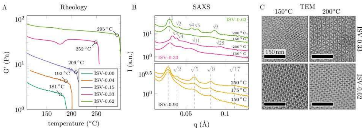
Figure 5. (A) Isochronal temperature scans data ( \omega = 1 rad/s, \gamma = 1\% , 2 °C/min) for ISV- x samples with T_{ODT} < 300 °C. (B) Selected SAXS data for the samples ISV-0.33, ISV-0.62 and ISV-0.9 which were annealed at various temperatures. (C) Selected TEM images for the samples of ISV-0.33 and ISV-0.62 which were annealed at different temperatures. Typical absolute values of G' and G'' are provided in Supporting Information, SI5, for ISV-0.33.
