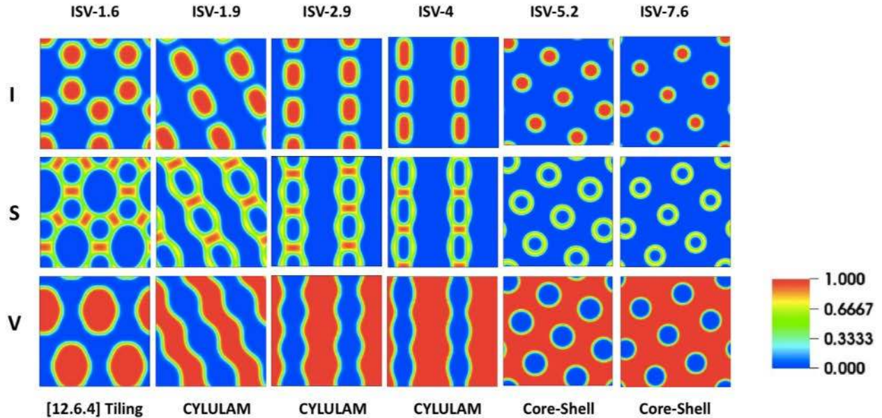
Figure 2. Detailed SCFT equilibrium volume fraction distribution of I, S and V as a function of x , where x is the volume ratio of V over I (volume of I and S are kept fixed for all the samples and they are equal to each other). Here x is varied between 0 and 7.6. Starting with lamellar profile for IS, the morphology evolved into 3 lamellar (ISV-0.04 and ISV-0.15) , [12.6.4] tiling (ISV-0.33) , [8.6.6; 8.6.4] tiling (ISV-0.43) , [8.8.4] tiling (ISV-0.62 and ISV-0.9) , [12.6.4] tiling (ISV-1.6), cylinders in undulating lamellae (CYLULAM) (ISV-1.9, ISV-2.9 and ISV-4) and finally to core-shell structure (ISV-5.2 and ISV-7.6) as the volume ratio of V over I is gradually increased from 0 to 7.6. For ISV-0.04 to ISV-0.33, V is miscible in S but for the other samples, it segregates into its own distinct domain. The color bar for volume fraction at the bottom right is shown for reference. The volume fraction of the three different components are not binary (the volume fraction is not zero or unity at any grid) as one would get an impression from SCFT images presented in Figure 1, the interfaces between the different components are smooth.
