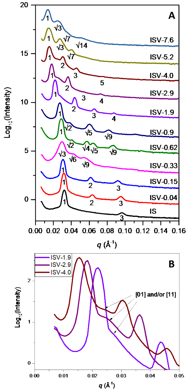
Figure 3. (A) SAXS results for ISV- x samples; annealing temperature is 150 °C for 0 \leq x \leq 0.33 , 200 °C for x = 0.62 and 175 °C for the rest. The scattering peaks are consistent with the real space morphologies obtained using TEM. (B) Zoom in of the [01] and/or [11] peak for the samples: ISV-1.9, ISV-2.9 and ISV-4.
