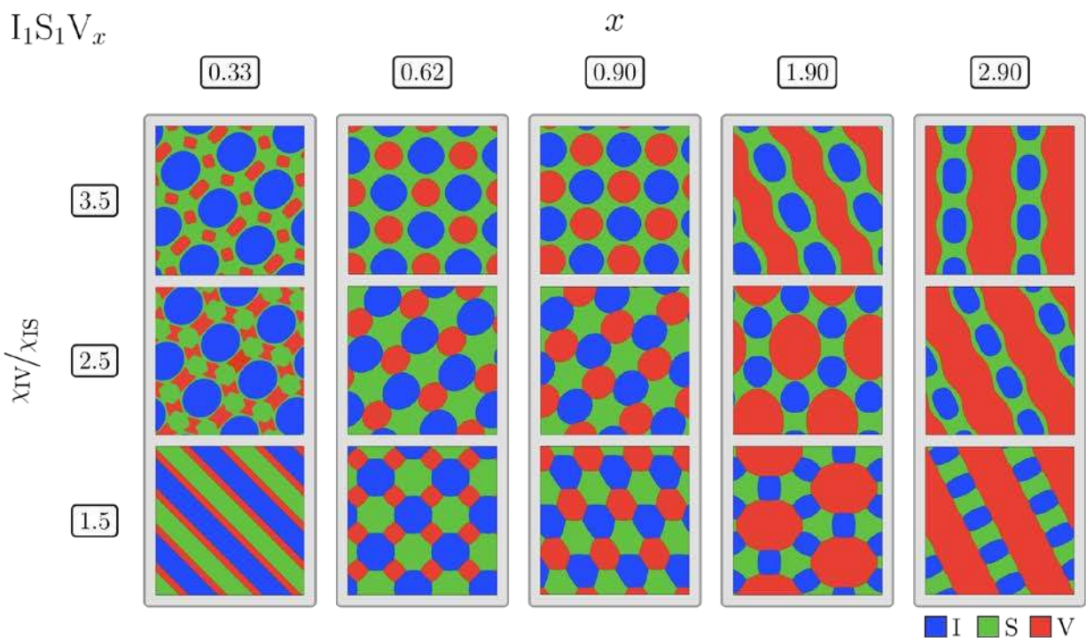
Figure 6. SCFT studies on the effect of \chi_{IV}/\chi_{IS} on the morphology of five different samples of ISV- x for qualitatively simulating the morphological changes. The morphology for ISV-0.33 changed from [12.6.4] tiling structure to LAM-3 as \chi_{IV}/\chi_{IS} is reduced from 3.5/2.5 to 1.5, morphology for ISV-0.62 changed from [8.8.4] tiling to [6.6.6] tiling to [8.8.4] tiling as \chi_{IV}/\chi_{IS} is changed from 3.5 to 2.5 to 1.5. The morphology for ISV-0.9 changed from [8.8.4] tiling to [6.6.6] tiling as \chi_{IV}/\chi_{IS} is reduced from 3.5/2.5 to 1.5, both ISV-1.9 and ISV-2.9 formed CYLULAM structure at \chi_{IV}/\chi_{IS} = 3.5 but with reduction of \chi_{IV}/\chi_{IS} to 2.5/1.5 ISV-1.9 formed [12.6.4] tiling structure, whereas ISV-2.9 retained its CYLULAM structure for \chi_{IV}/\chi_{IS} = 2.5 and transformed to ALT.LAM when \chi_{IV}/\chi_{IS} was further lowered to 1.5. For all the cases, the dominating volume fraction of the component (I or S or V) was used to represent that particular grid point except for ISV-0.33. For ISV-0.33, the dominant of I or S or if the volume fraction of V is greater than a cut-off value (from top to bottom the cut-off values are: 0.25, 0.22 and 0.2031) was used to represent the grid point. Color code: blue I, green S, red V. (See SI6 for detailed equilibrium volume fraction profiles of all three components)
