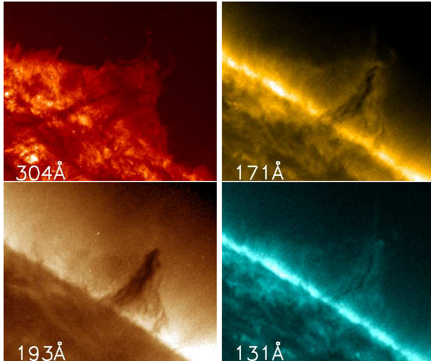
Fig. 1.— SDO/AIA images of a quiescent prominence observed at 15:38 UT on the limb on 22 June 2010 over a 124'' \times 108'' field of view. From top left to bottom right: single exposure for 304 band ( \log T = 4.7 ), 171 band ( \log T = 5.8 ), 193 band ( \log T = 6.1 ) and 27 sec exposure for 131 band ( \log T = 5.8 and 7).
