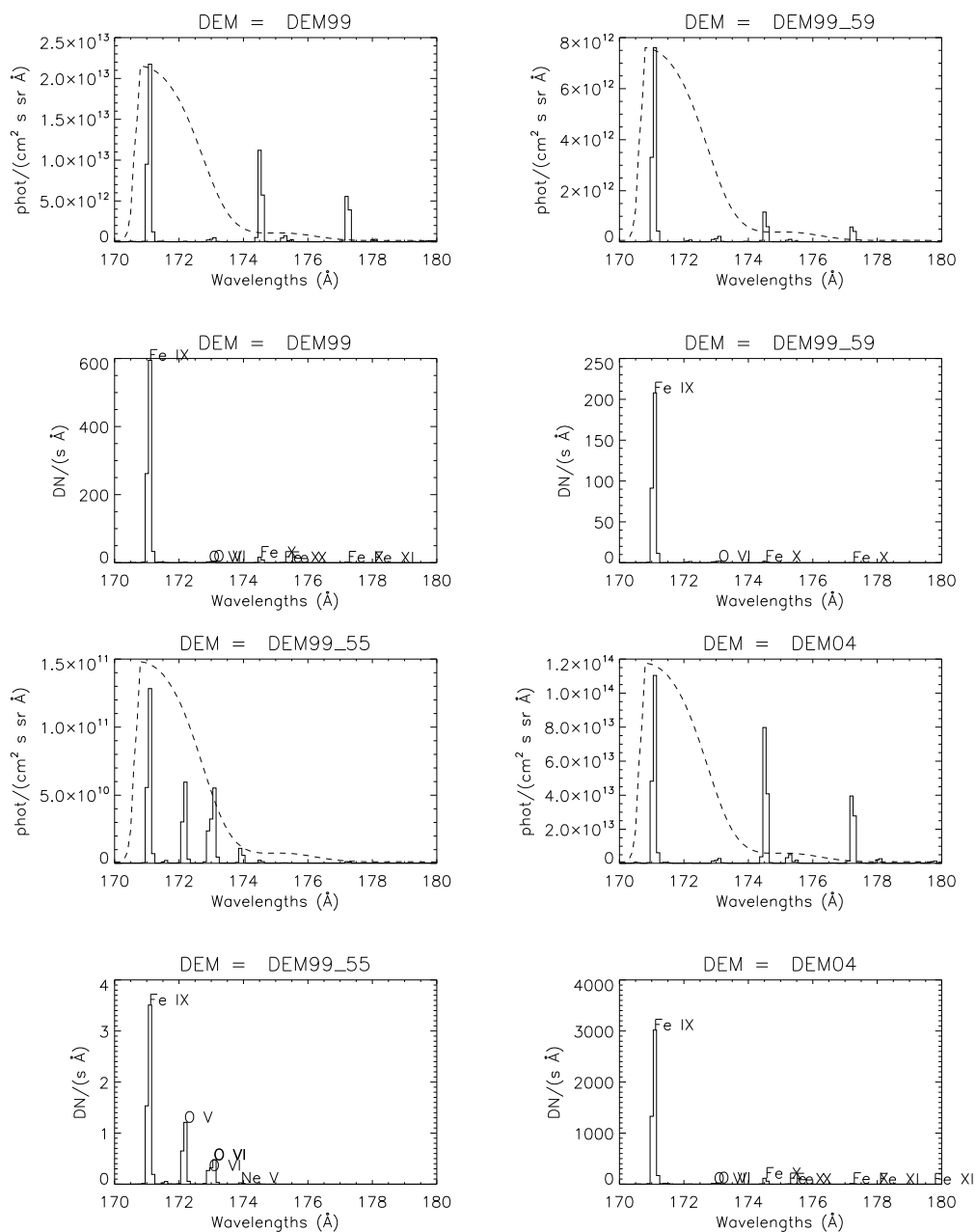
Fig. 6.— Synthetic CHIANTI spectrum contributing to the AIA 171 band derived using the different prominence DEMs plotted in Figure 5. For each DEM the top panel shows the prominence spectrum with superimposed the effective area of the AIA filter. The bottom panel shows the spectrum predicted to contribute to the AIA bands obtained by the product of the spectrum shown in the top panel with effective area of the instrument.
