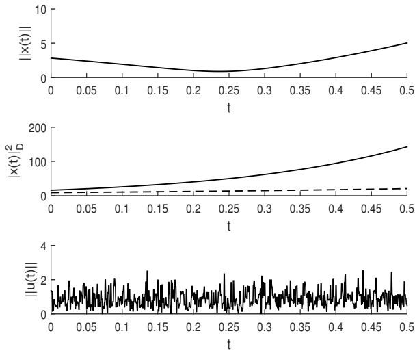
Fig. 4. The time plots of \|x(t)\| , |x(t)|_{\mathcal{D}}^2 , and \|u(t)\| with initial state x_0 = (2, 2) . The dashed curve in the middle plot shows the lower-bound of |x(t)|_{\mathcal{D}}^2 such that the safety of (21) is still preserved in the presence of disturbance u .
