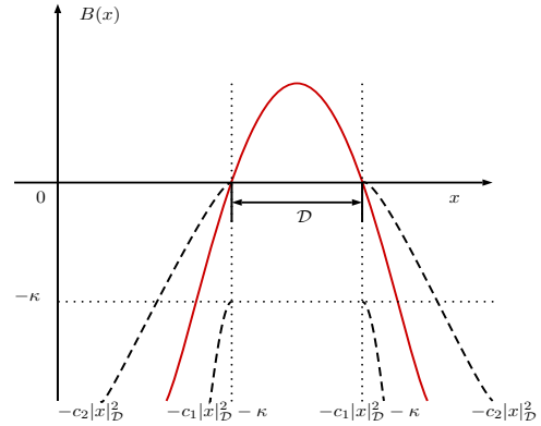
Fig. 2. An illustration of a practical ISSf barrier function which takes the form of a quadratic function, e.g., B(x) = -(x - x^*)^T P (x - x^*) + c where P is a positive definite matrix, x^* is the centroid of the unsafe set \mathcal{D} and c is a constant that is chosen such that the zero level of B is equal to the boundary of \mathcal{D} . The solid red-line is the plot of B and the dashed-line shows the possible lower and upper bound of B using the set distance function |x|_{\mathcal{D}} and a bias constant \kappa > 0 as used in Proposition (1), c.f., (13).
