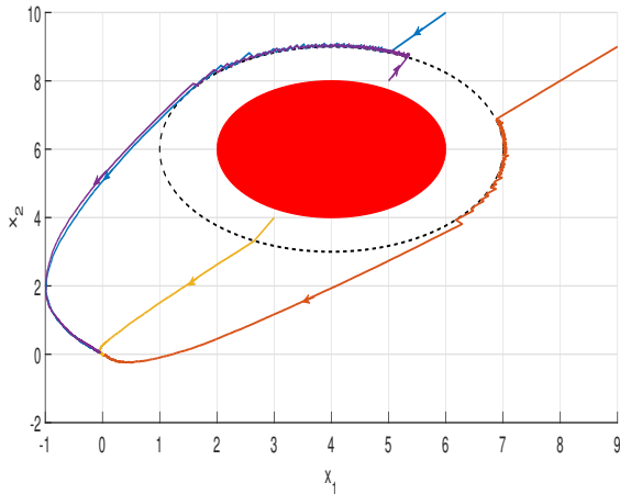
Fig. 5. State trajectories x(t) discussed in Example 2, starting from four different initial conditions. The set of unsafe state \mathcal{S} is shown in red area, and the boundary of \mathcal{X} is shown by dashed line.
