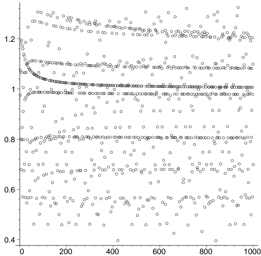
Figure 2: The function m \mapsto \pi_m
