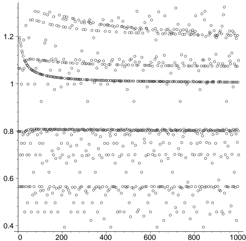
Figure 1: The function m \mapsto \kappa_m
