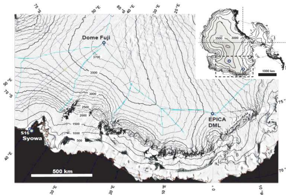
Figure 1. The Atlantic sector of the East Antarctic ice sheet with the positions of Dome Fuji (DF) and the EPICA Dronning Maud Land (EDML) drilling sites. Black lines are elevation curves in metres, blue curves indicate major ice flow lines, and the grey lines are traverse tracks. Satellite image from MODIS (Haran et al., 2005, updated 2006).
