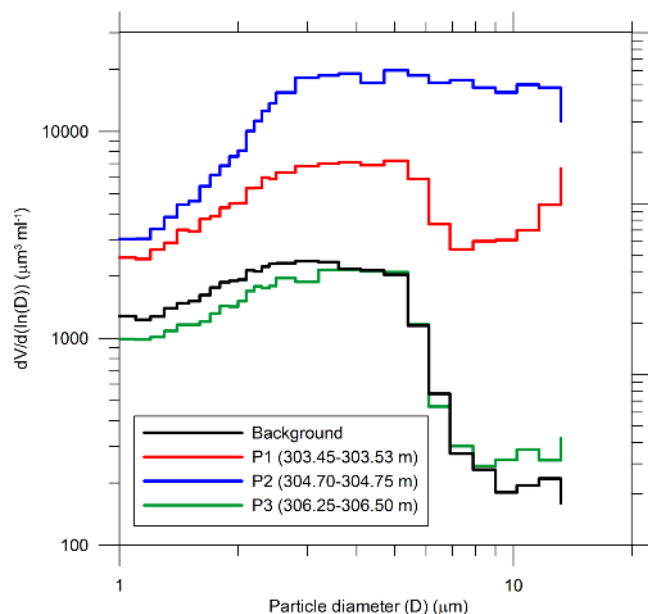
Figure 6. Dust volume distributions of average background dust and across the three prominent volcanic peaks, P1, P2, and P3 (see Fig. 2). The size distributions are obtained by an Abakus instrument that covers the particle size interval 1–15 \mu\text{m} (spherical equivalent diameter). The Abakus is known not to measure dust sizes as accurately as a Coulter counter instrument (Ruth et al., 2003), and the shape of the dust size distribution may be somewhat biased. The relative sample differences in dust sizes are, however, robust and significant.
