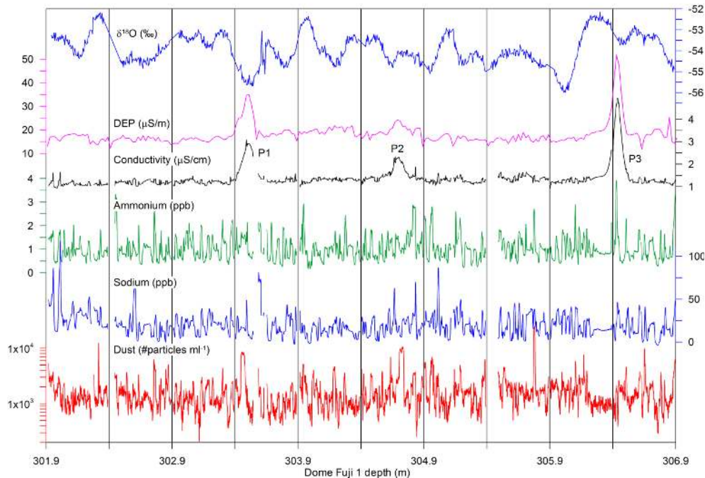
Figure 2. Overview of the high-resolution records obtained from the 5 m of early Holocene Dome Fuji ice. From the top, the \delta^{18}\text{O} is obtained continuously on a cavity ring-down spectrometer and the dielectric profiling (DEP) is made on the solid ice. The electrolytic conductivity, the ammonium, the sodium, and the dust concentrations were obtained on the Copenhagen CFA analytical system. Data gaps are due to core breaks or failure of the analytical systems. The three major acidity spikes P1, P2, and P3 centred at 303.51, 304.70, and 306.44 m depth, respectively, are indicated.
