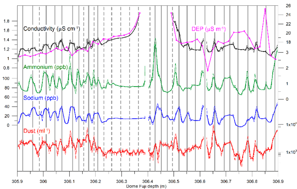
Figure 4. Same records as shown in Fig. 3 plus the DEP record for the section containing the major acidity peak P3 centred at around 306.44 m depth and the “peculiar event” with unusually smooth profiles 306.25–306.40 m depth. Thin curves show the records at a 1 mm depth resolution and thicker curves are 1 cm averages. “Certain” and “uncertain” annual layer marks are indicated with full and dashed vertical lines, respectively. For the interval 306.25–306.40 m the layer indication is tentative.
