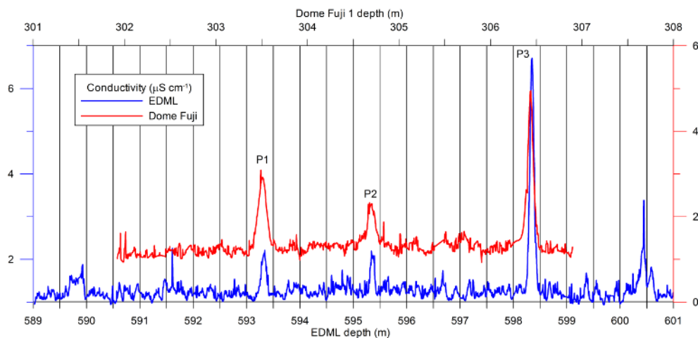
Figure 5. Volcanic matching of the Dome Fuji and EPICA Dronning Maud Land (EDML) ice cores based on the three characteristic acidity peaks P1, P2, and P3, here shown in the electrolytic conductivity signal. Due to the different shapes of the acidity peaks, the matching of the cores has an uncertainty of a few years.
