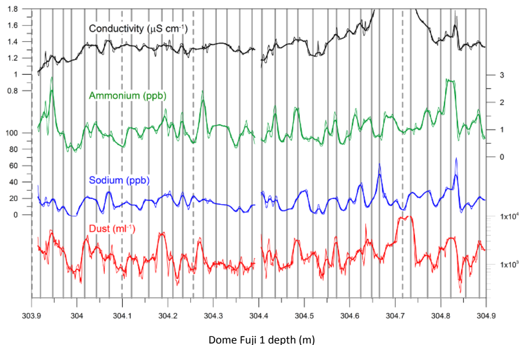
Figure 3. Example of high-resolution profiles of electrolytic conductivity, ammonium, sodium, and dust concentrations. Thin curves show the records at a 1 mm depth resolution and thicker curves are 1 cm averages. “Certain” and “uncertain” annual layer marks are indicated with full and dashed vertical lines, respectively. The entire data set is shown in the Supplement Figs. S1–S5.
