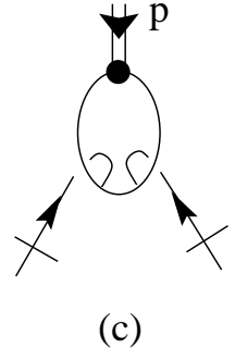
Figure 2: One-loop insertion in 1PI two-point function.
