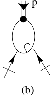
Figure 2: One-loop insertion in 1PI two-point function.
