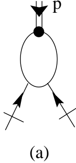
Figure 2: One-loop insertion in 1PI two-point function.
