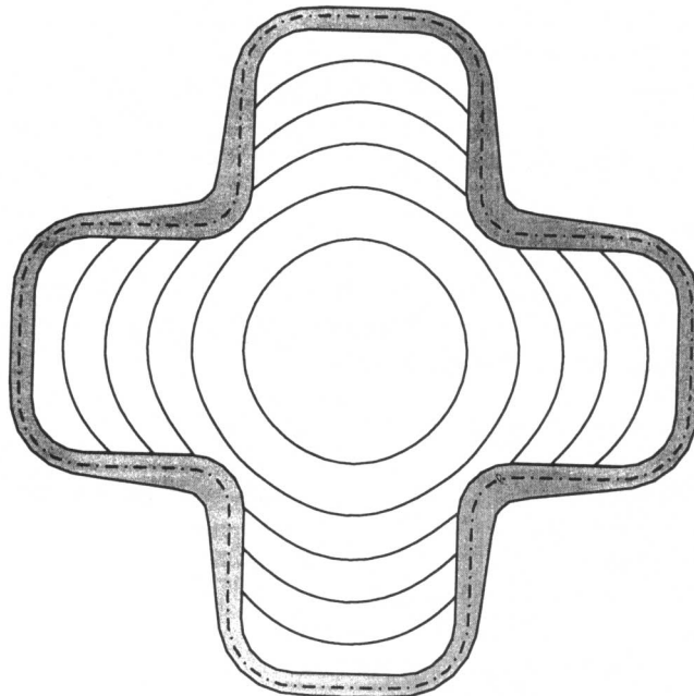
Fig. 3. Best insulation of a cross.
