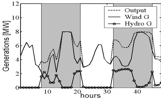
Fig. 4. W-H Operation – Case (A) – Average Output, Wind and Hydro Active Power Generations
