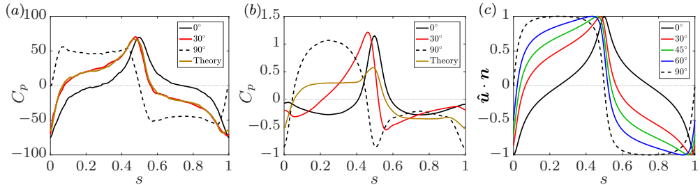
Figure 6: Distribution of C_p against normalized distance s along the circumference of the meridional section for (a) Re = 0.1 and (b) Re = 100 ; (c) surface normal projections \hat{\mathbf{u}} \cdot \mathbf{n} for different incident angles \phi . Note the linearity theory matches perfectly with simulations for Re = 0.1 and shows strong mismatch for Re = 100 . For the different \phi shown, note the matching trends of C_p at Re = 0.1 with \hat{\mathbf{u}} \cdot \mathbf{n} .
