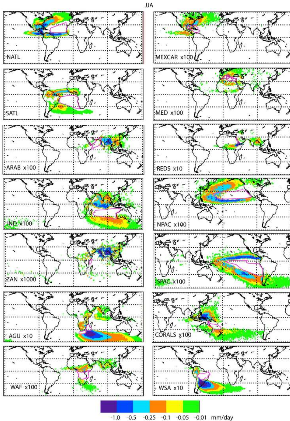
Figure 3. The same as Figure 2, but for JJA.
