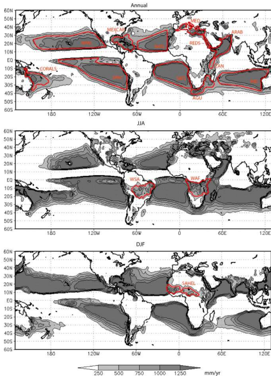
Figure 1. Climatological (top) annual, (middle) JJA and (bottom) DJF vertically integrated moisture flux divergence (mm/yr). Values higher than 250 mm/yr are in gray scale, with an interval between isolines of 250 mm/yr. Areas inside the red contour lines indicate the regions considered as moisture sources in the forward integrations. The areas were defined based on the threshold of 750 mm/yr for the oceanic sources (CORALS, Coral Sea; NPAC, North Pacific; SPAC, South Pacific; MEXCAR, Mexico Caribbean; NATL, North Atlantic; SATL, South Atlantic; ARAB, Arabian Sea; ZAN, Zanzibar Current; AGU, Agulhas Current; IND, Indian Ocean) and 500 mm/yr for the land sources (WAF, Winter Africa; WSA, Winter South America; SAHEL, Sahel). Two boxes were also defined using the physical boundaries of oceanic basins (MED, REDS). Data: ERA40 (1958–2001).
