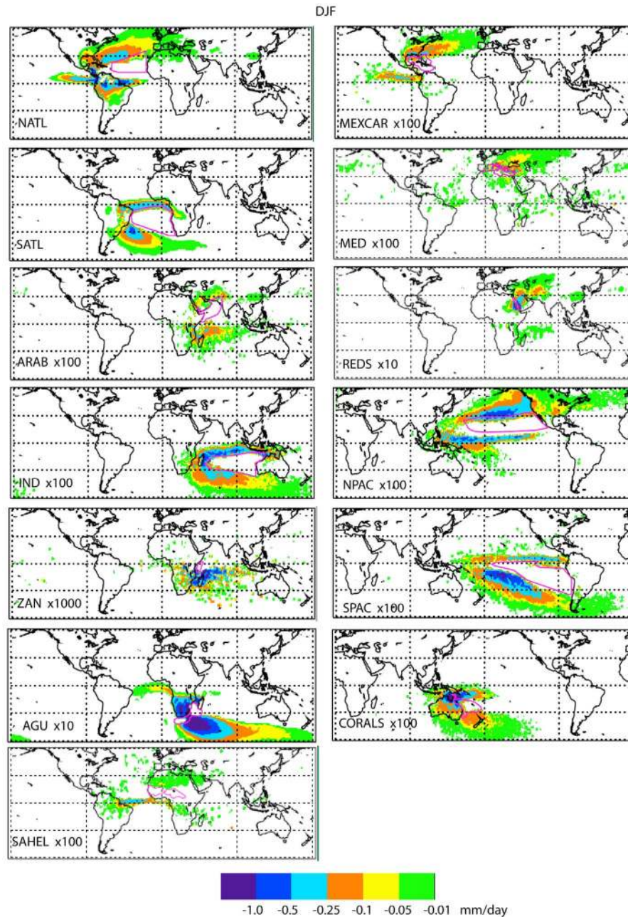
Figure 2. DJF fields of (E-P) integrated over 10 days for the period 2000–2004 calculated by forward tracking from the moisture sources indicated by the pink lines and identified on the left bottom of each plot. Only negative values are plotted and they were scaled by the different factors indicated in each plot in order to use the same colour bar.
