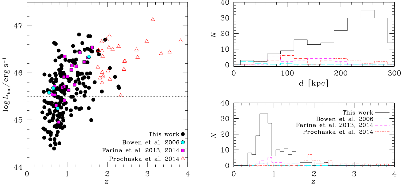
Figure 1. left: Bolometric luminosity of the foreground quasars versus foreground quasar redshift. The horizontal dotted line marks \log L_{\text{bol}} / \text{erg s}^{-1} = 45.5 , the division between the luminous and low-luminosity quasars used throughout the paper. right: Projected distance ( top ) and redshift ( bottom ) histograms. In all three panels, quasars from Bowen et al. (2006), Farina et al. (2013) or Farina et al. (2014), Prochaska et al. (2014), and this work are displayed in cyan, magenta, red, and black respectively, with symbols and line-styles indicated in the legend. The quasars from Bowen et al. (2006), Farina et al. (2013), Farina et al. (2014), and this work have available constraints on the transverse Mg II absorption from the spectra of background quasars. Mg II absorption constraints are unavailable for the quasar sample from Prochaska et al. (2014) due to the higher redshift range. For these quasars, C II rather than Mg II serves as a signature of cool, high HI column density gas.
