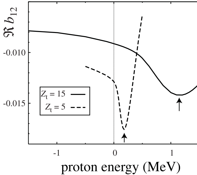
Fig. 8. The real part of b_{12} in ^{24}\text{S} ( Z_t = 15 , solid line). The dashed line shows results with the Coulomb potential reduced by a factor of three ( Z_t = 5 ). The turning points are marked by arrows.
