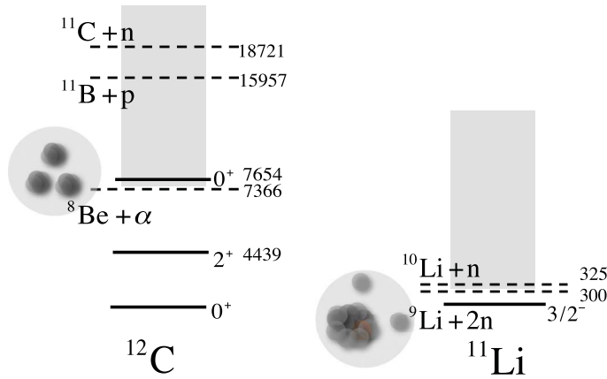
Fig. 1. Example of two Borromean systems: ^{12}\text{C} and ^{11}\text{Li} . The near-threshold states in these nuclei – the Hoyle resonance 0_2^+ in ^{12}\text{C} and the weakly-bound 3/2_1^- ground state in ^{11}\text{Li} – exhibit a strong imprint of the nearby decay threshold, i.e., ^{12}\text{C} \rightarrow ^8\text{Be} + \alpha and ^{11}\text{Li} \rightarrow 2n + ^9\text{Li} .
