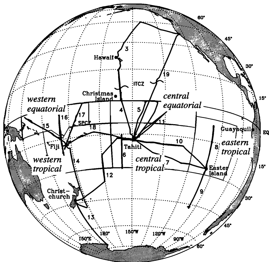
Figure 1. Flight tracks of the DC-8 aircraft during PEM-Tropics A. Thin solid lines delineate the regions discussed in the text. Aircraft crossings of the intertropical convergence zone (ITCZ) and the South Pacific convergence zone (SPCZ) are indicated by tilde symbols.
