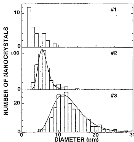
FIG. 1. The size distribution of Ge nanocrystals in SiO 2 matrix. The solid lines are log-normal functions.
