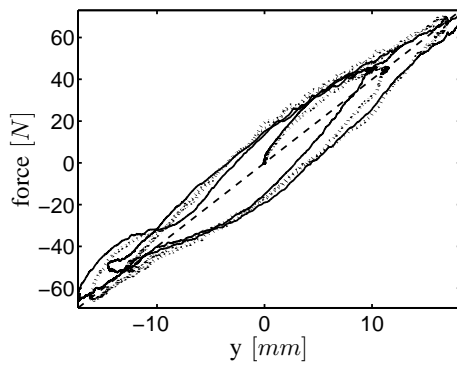
Fig. 9. Applied force vs. end-effector deviation in y -direction (solid line). The dashed line corresponds to the desired stiffness. The dotted line shows a (simplified) simulation result.
