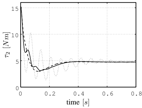
Fig. 5. Simulated joint torque for a step wise excitation of 10Nm (dotted line: B_\theta = B , solid line: B_\theta = B/3 , dashed line: B_\theta = B/10 ).
