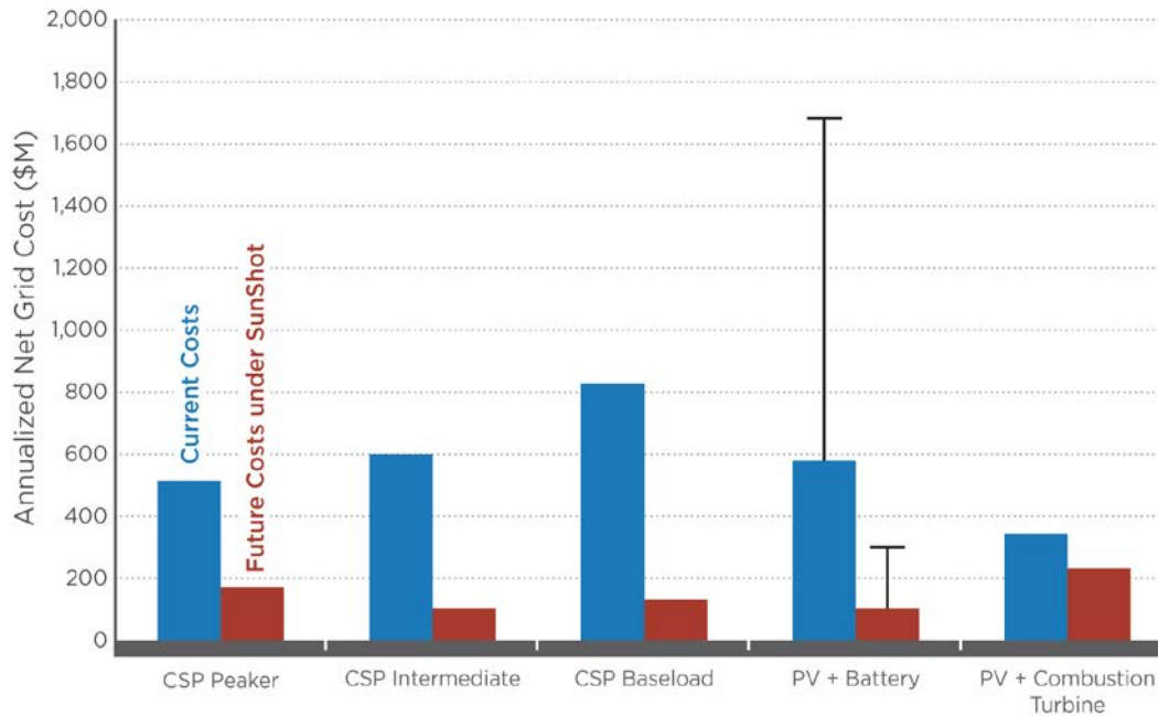
Figure 20. Annualized net cost results for analysis of current and future cost scenarios for CSP, PV with batteries, and PV with combustion turbines
