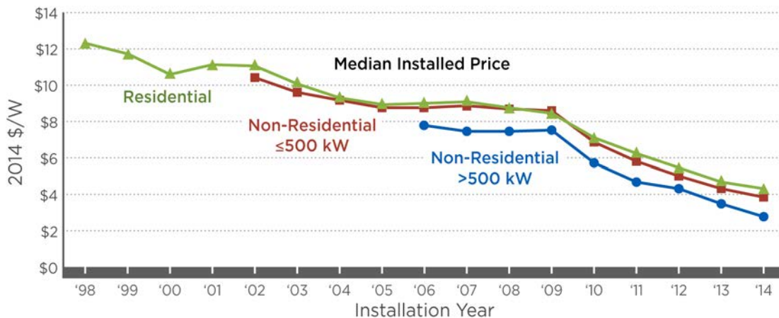
Figure 3. Falling prices of PV in 2014 dollars per watt for residential and non-residential markets
