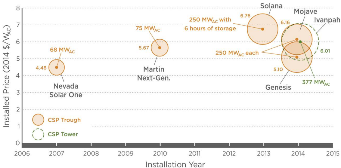
Figure 13. Historic installed costs for CSP projects in the U.S. from 2007 to 2014
