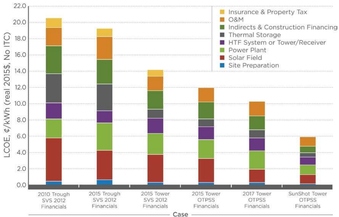
Figure 16. Cost category contributions to LCOE for the cases shown in Table 6
