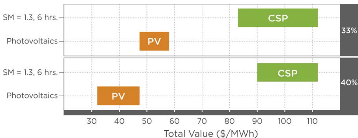
Figure 5. Total value, which includes operational and capacity value, of CSP-TES and PV under 33% and 40% RPS scenarios
