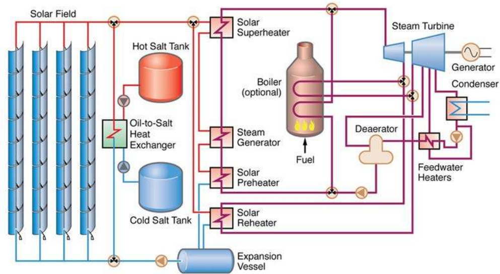
Figure 7. Parabolic trough plant with indirect two-tank thermal storage and fossil-fuel backup system
