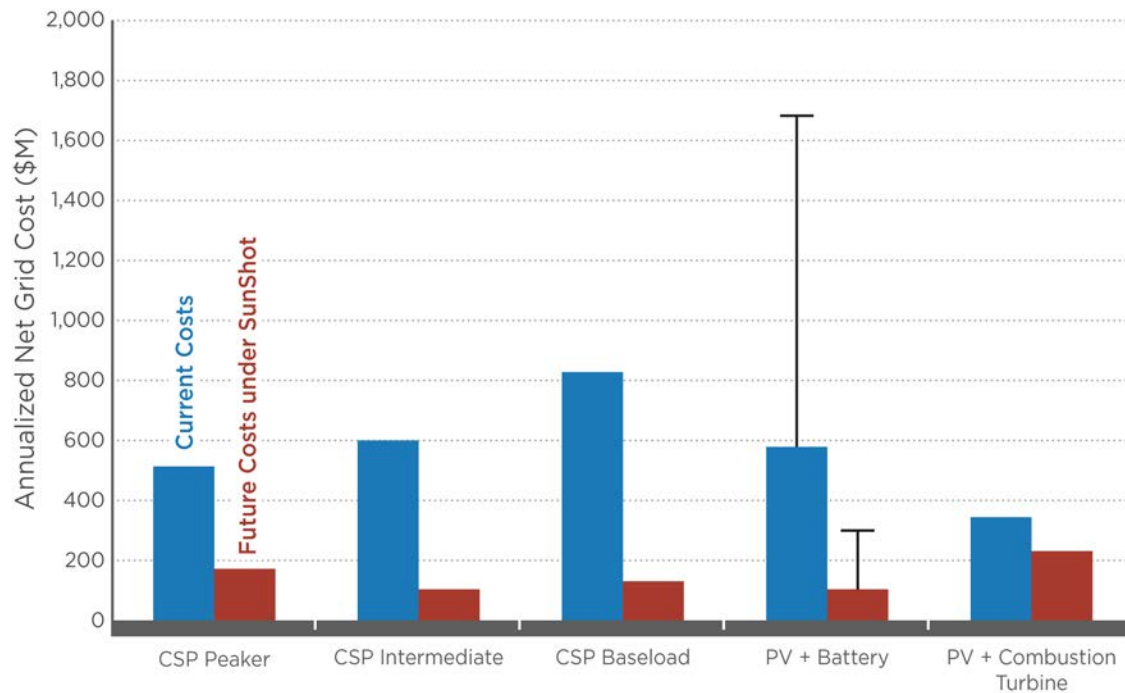
Figure ES-4. Annualized net cost results for analysis of current and future cost scenarios for CSP, PV with batteries, and PV with combustion turbines
