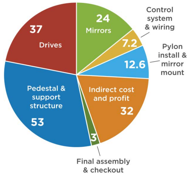
Figure 15. Cost breakout ($/m 2 ) for the LH-2.2 heliostat used to update NREL’s molten-salt power-tower model
