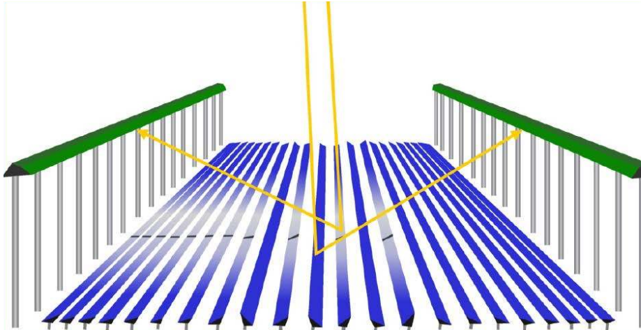
Figure 11. Compact linear Fresnel system
