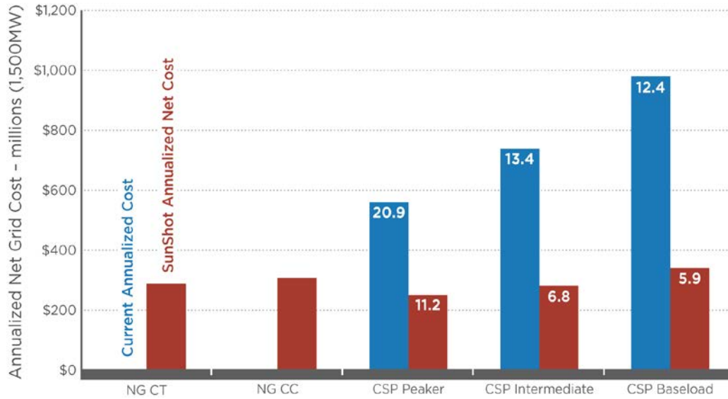
Figure 17. Comparison of annualized net cost of current and SunShot CSP configurations (peaker, intermediate, baseload) and conventional combustion turbine and combined-cycle plants assuming low natural gas and emission cost scenarios
