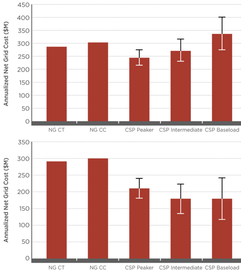
Figures ES-3. Low natural gas and emission cost scenario (top) and high natural gas and emissions cost scenario (bottom)
