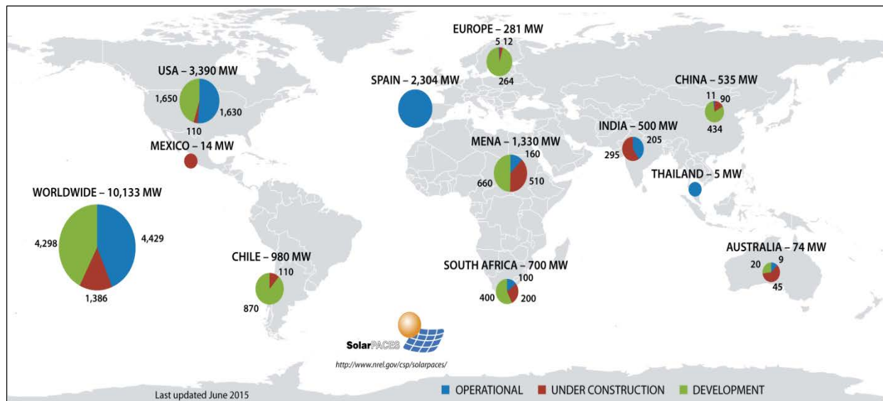
Figure 2. Cumulative CSP capacity by country and status (operational, under construction, development)
