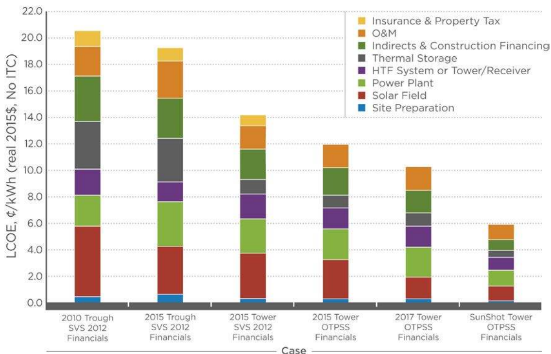
Figure ES-1. Cost reductions for parabolic trough and tower technologies since the SunShot Vision Study
