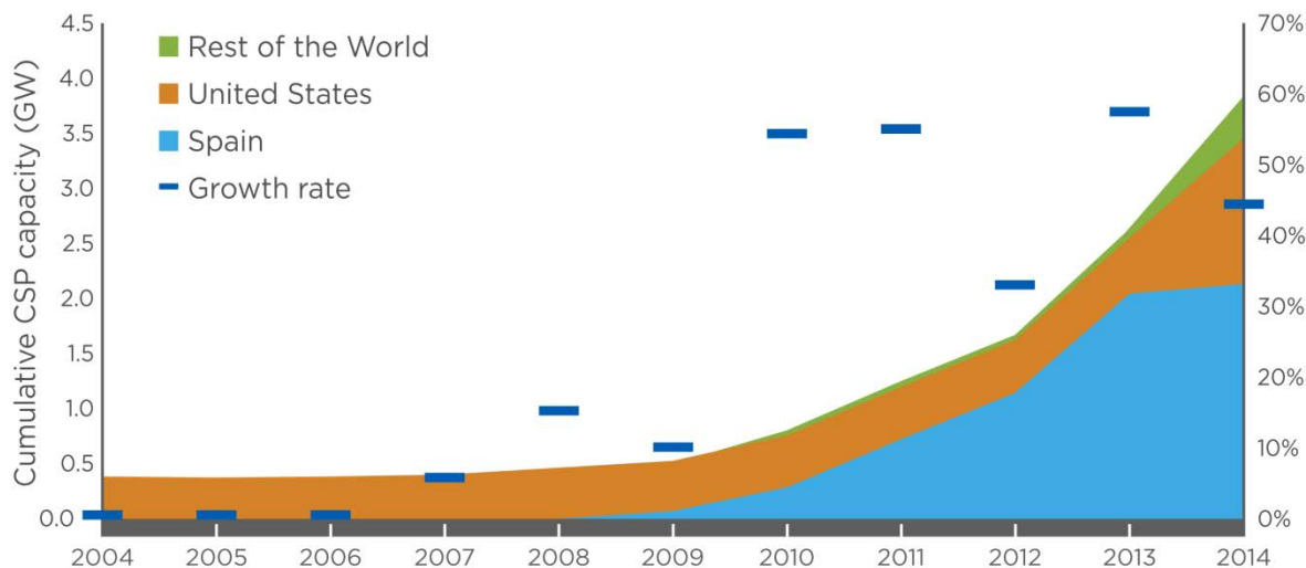
Figure 1. Global cumulative growth of CSP capacity
