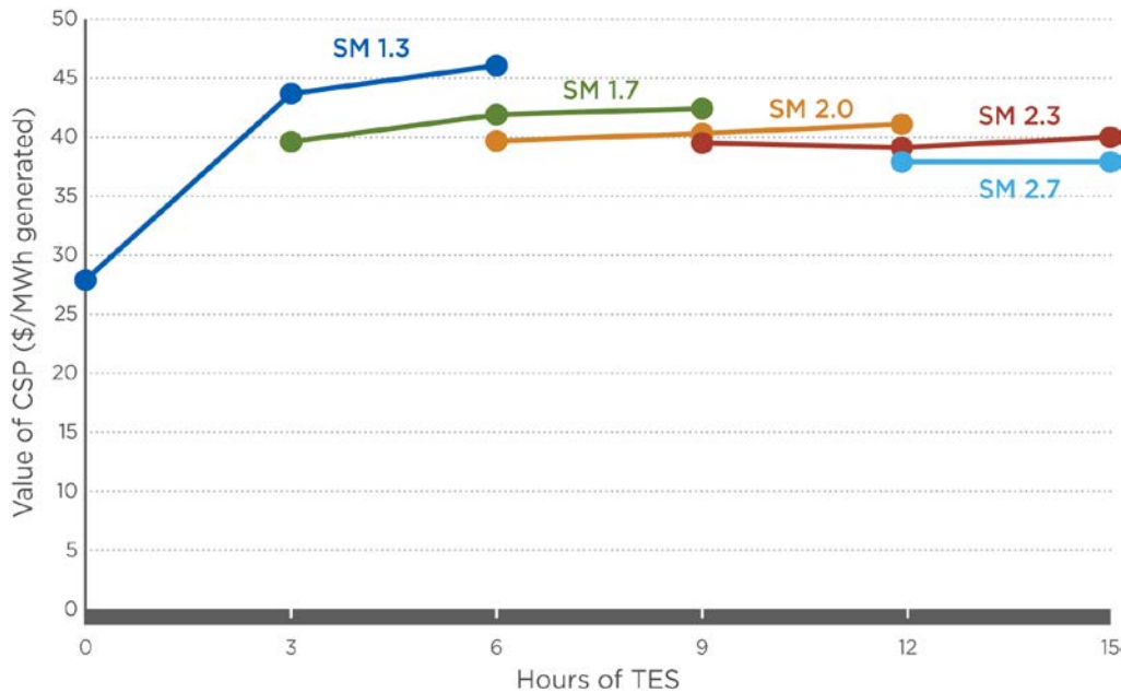
Figure 4. Marginal operational value of tower CSP-TES plants with varying configurations in California
