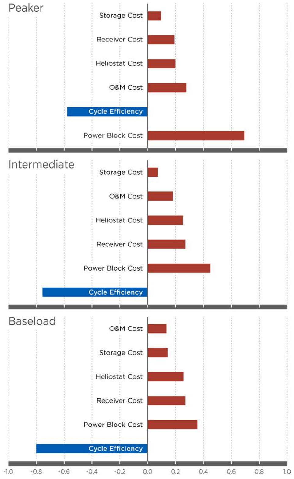
Figure 19. Standardized rank-order coefficients for peaker, intermediate, and baseload CSP configurations
