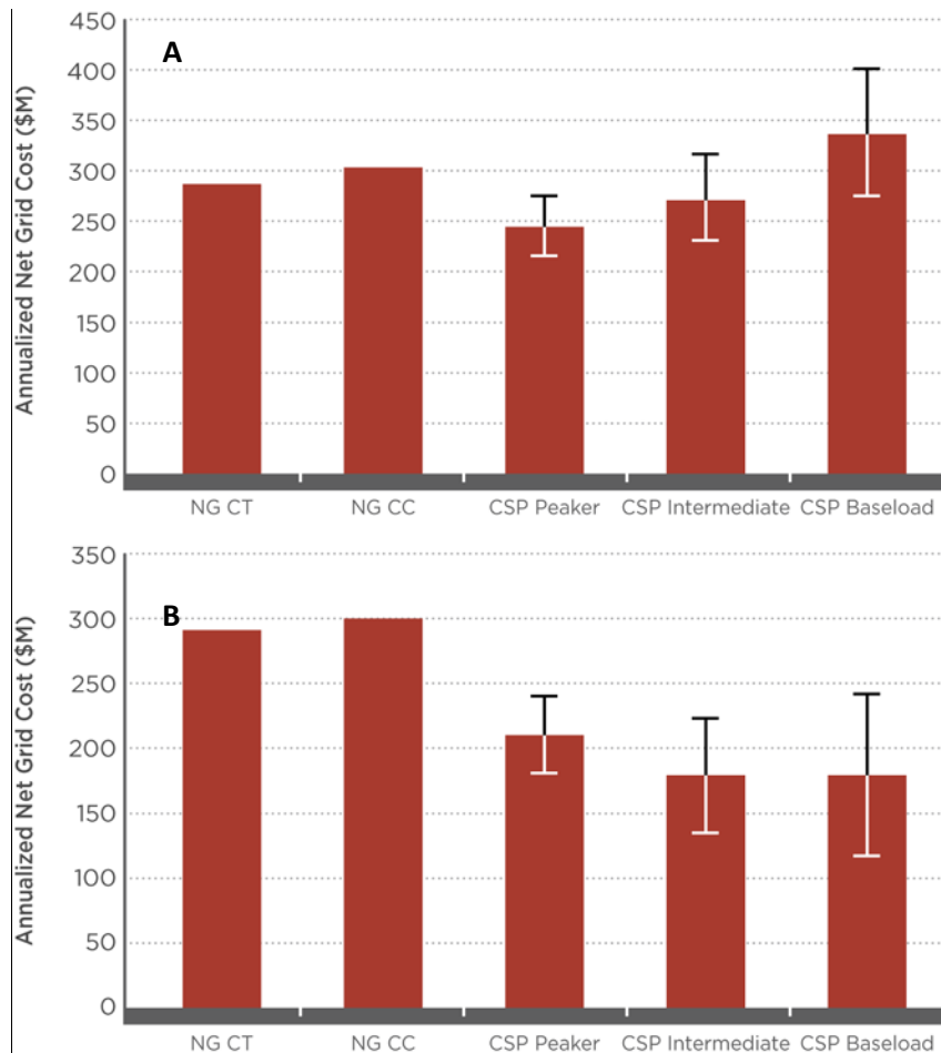
Figures 18. Low natural gas and emission cost scenario (A) and high natural gas and emissions cost scenario (B)
