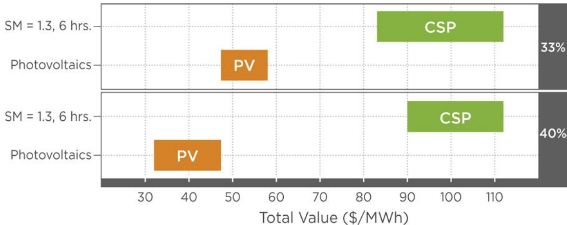
Figure ES-2. Total value, which includes operational and capacity value, of CSP with thermal energy storage and PV under 33% and 40% RPS scenarios
