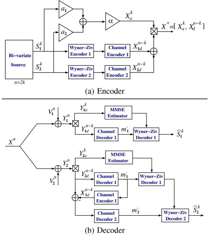
Fig. 3. Broadcasting a bivariate source S^k = (S_1^k, S_2^k) with bandwidth expansion: the HWZ scheme.
