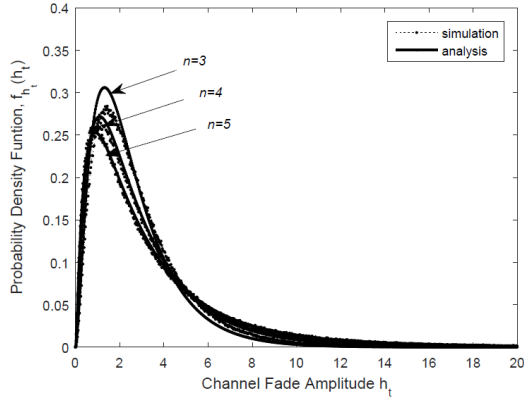
Fig. 1. Comparison between analytical results and Monte-Carlo simulation for the PDF formulated by (3) ( n = 3; m = 2.256, \Omega = 1.424 ), ( n = 4; m = 2.87, \Omega = 1.351 ), ( n = 5; m = 3.477, \Omega = 1.306 ), \sigma^2 = 1, L = 2 and 10^6 iterations.
