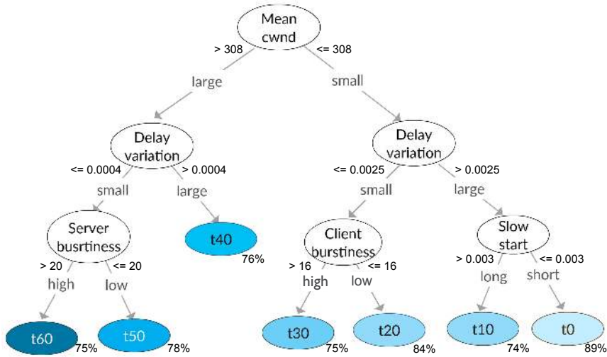
(b) Learned decision tree for QUIC.
