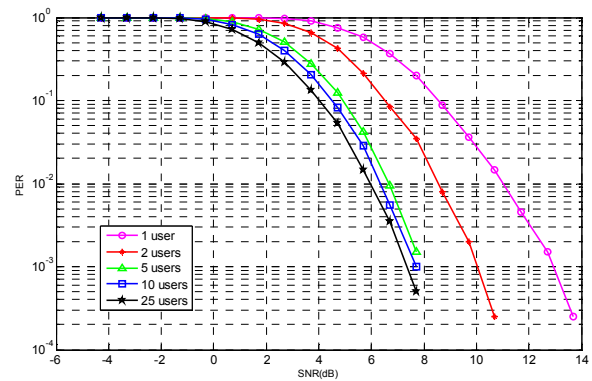
Figure 9: PER Performance of SU-MIMO SM with different numbers of users
