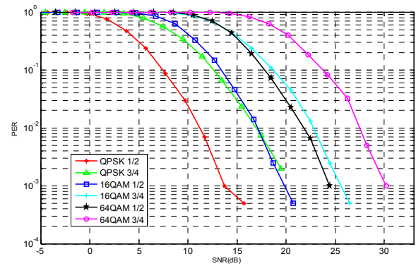
Figure 2: SISO PER Performance for Urban Macro channel
