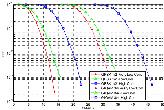
Figure 6: MIMO 2x2 SM PER Performance for QPSK \frac{1}{2} rate with different correlation factors
