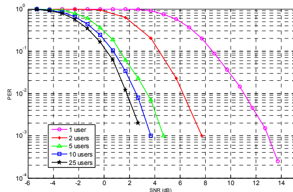
Figure 10: PER Performance of MU-MIMO SM with different numbers of users
