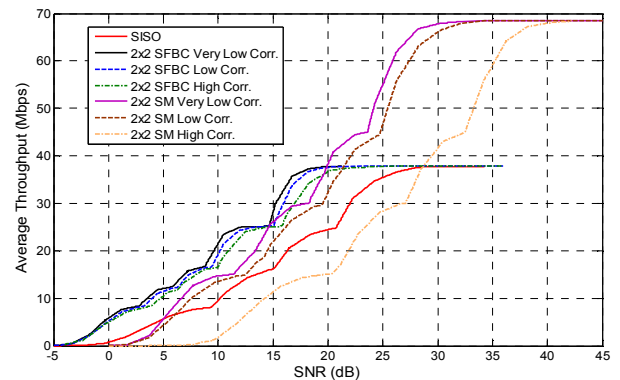
Figure 11: Average Throughput of SISO, MIMO 2x2 SM and MIMO 2x2 SFBC with different correlation factors
