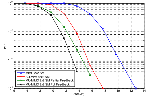
Figure 8: PER performance of SU-MIMO and MU-MIMO SM
