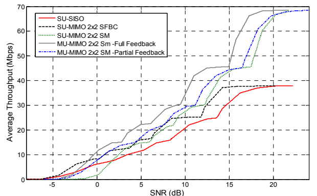
Figure 12: Average Throughput of SISO and MIMO schemes with frequency domain allocation at very low correlation channels
