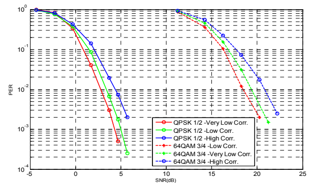
Figure 4: MIMO 2x2 SFBC PER Performance for QPSK \frac{1}{2} rate and 64QAM \frac{3}{4} rate with different correlation modes
