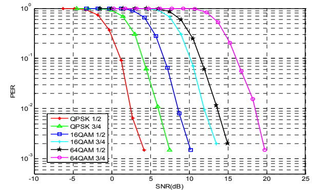
Figure 3: MIMO 2x2 SFBC PER Performance for Urban Macro channel with very low correlation (0.1)
