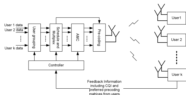
Figure 1: Configuration of MU-MIMO System
