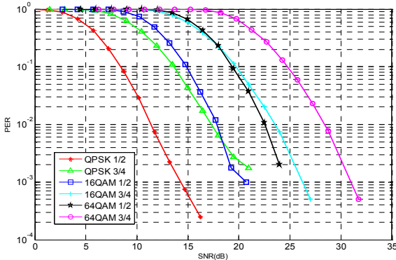
Figure 5: MIMO 2x2 SM PER Performance for Urban Macro channel with very low correlation (0.1)
