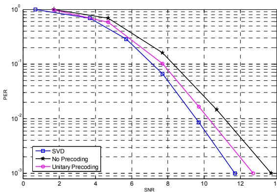
Figure 7: PER Performance of 2x2 SM with unitary precoding
