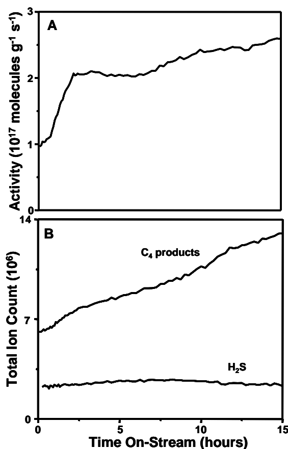
S. I. Figure 1: (A) Thiophene HDS activity measurement for pretreated Ni 3 B as a function of time at 450 °C. (B) Product formation as a function of time on stream at 450 °C for Ni 3 B.
