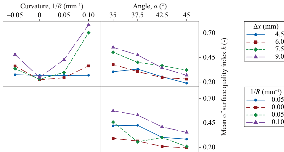
Figure 9 Interaction plot for the surface quality index k (see online version for colours)
