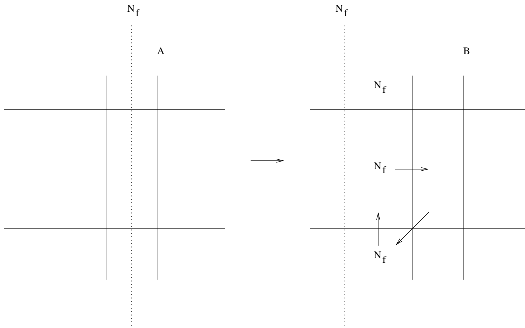
Figure 7: The creation of various boxes of D5-branes when a D7-brane and an NS-brane cross. The case with a single finite box. The arrows indicate all possible chiral fields relevant to the interaction between the D7-brane and the D5-branes.
