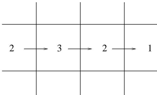
Figure 9: The (3,2) model SU(3) \times SU(2) without superpotential.
