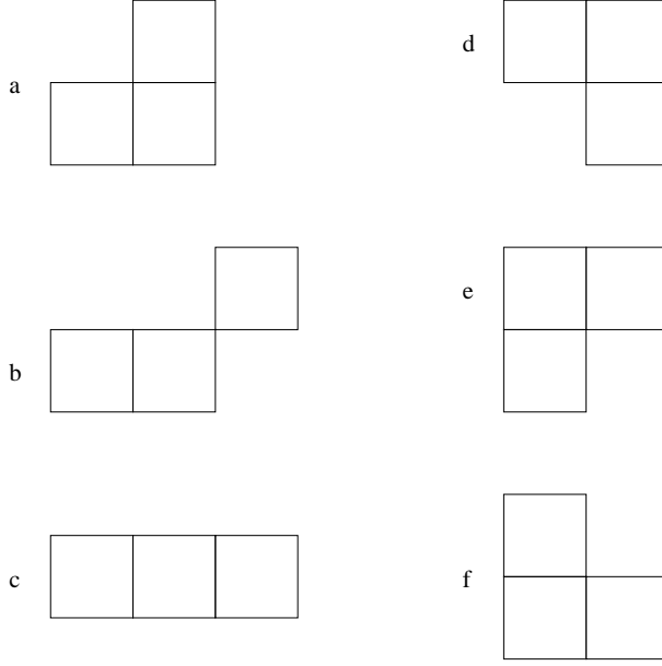
Figure 10: Various cases of three-box models.
