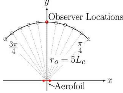
FIGURE 6. A circular arc of observer locations (a virtual microphone array) used for the calculation of radiated sound power based on (3.1).
