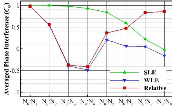
FIGURE 23. Averaged phase-interference levels of surface pressure fluctuations along the LE between the Peak ( N_0 ) and the remaining probe points ( N_1, \dots, N_8 ) obtained by integrating the profiles shown in figure 22. The definition of C_\Phi is given in (4.2).
