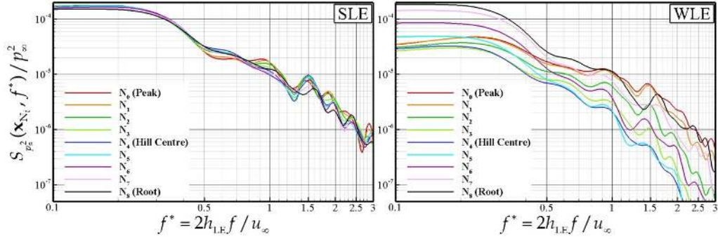
FIGURE 16. Auto-spectra of surface pressure fluctuations along the LE; S_{p'_s}(\mathbf{x}_{N_i}, f) for i = 0, \dots, 8 ; obtained at the probe points denoted in figure 15, for the SLE (left) and WLE (right) cases. The WLE case is for h_{LE}/L_c = 1/15 and \lambda_{LE}/L_c = 2/15 .
