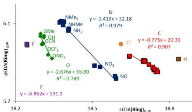
Fig. 11 Dependence of pEDA(Ring) on sEDA(Ring) for meta - and para -substituted nitrobenzene derivatives. For red points the sequence is Me, CN, CF 3 , CONH 2 , COOH, COMe, COCl, CHO. Reprinted with permission from J Phys Chem A 121:5196 (2017) [117]. Copyright 2017 American Chemical Society
