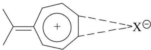
Scheme 5 Structure of heptafulvene-halogen atom complex ( X = \text{F}, \text{Cl}, \text{Br}, \text{I}, \text{At} ).
