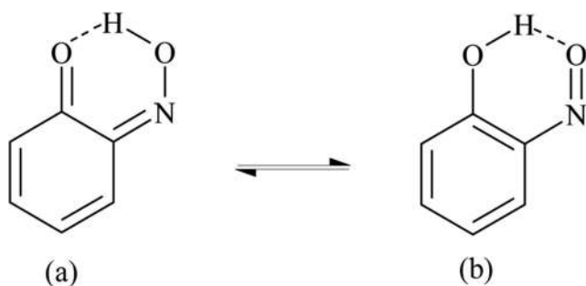
Scheme 11 Tautomeric equilibria in o -nitrosophenol: a ketoxime and b nitrosoenol forms
