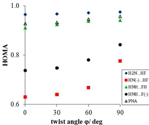
Fig. 12 Dependences of HOMA values on rotation angle \phi of NO 2 group in para -nitroaniline complexes (for equilibrium structures, except for HNH...F - interactions). Reused from Crystals 6:29 (2016) [148], this work is licensed under the Creative Commons Attribution 4.0 International License ( http://creativecommons.org/licenses/by/4.0/ )
