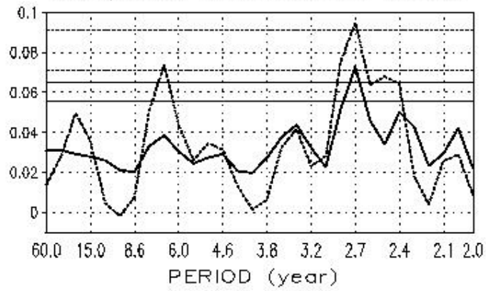
Power Spectrum of All Indian Rainfall Index, White Noise
