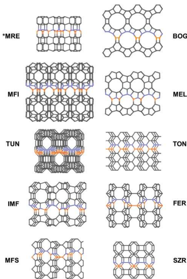
Fig. 4: The 3D framework structures of the ten butterfly family of zeolites viewed along the a -axis for *MRE , TON , IMF , FER , MFS and SZR , along the b -axis for BOG , MFI and MEL , and along [101] for TUN . The c -axis is vertical for all structures. Only the T–T connections (T = Si, Al) are shown for clarity. One butterfly layer is highlighted in each structure, with the T-atoms pointing up in blue and those pointing down in gold.
