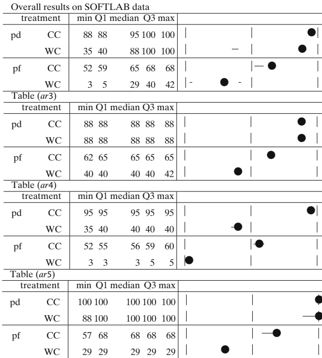
Fig. 12 Analysis #1 results for the SOFTLAB projects. Overall and individual results are shown respectively
