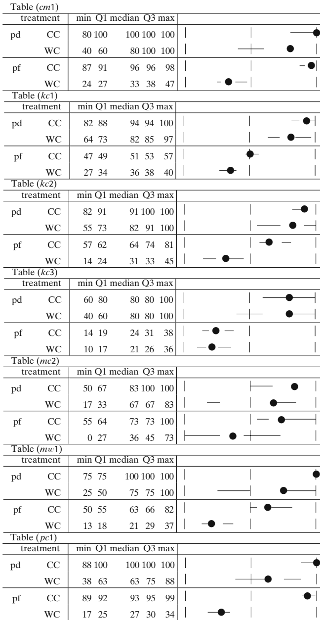
Fig. 5 Project-wise Analysis #1 results for NASA projects
