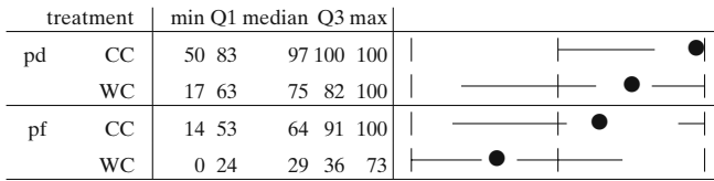
Fig. 4 Analysis #1 results averaged over seven NASA tables. Numeric results on left ; quartile charts on right . Q1 and Q3 denote the 25% and 75% percentile points (respectively). The upper quartile of the first row is not visible since it runs from 100% to 100%; i.e. it has zero length
