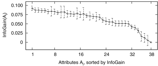
Fig. 3 InfoGain for KC3 attributes. Calculated from Eq. 2. Lines show means and t -bars show standard deviations after 10 trials on 90% of the training data (randomly selected)
