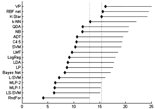
Fig. 16 x-axis shows the rank of the data miners given in the y-axis. All the methods whose top ranks are 4 to 12 are statistically insignificant different. From Lessmann et al. (2008)
