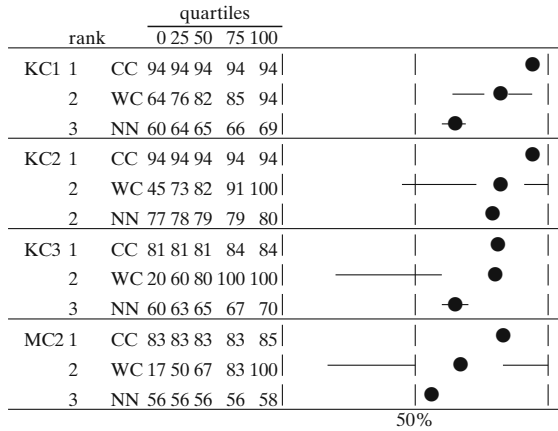
Fig. 7 Analysis #2 PD results where NN_{pd} < WC_{pd}
