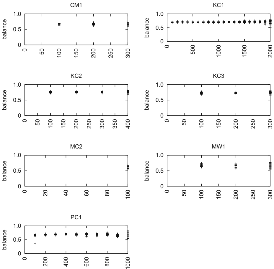
Fig. 10 Results from Analysis #3. Training set size grows in units of 100 examples, moving left to right over the x-axis. The MC2 results only appear at the maximum x-value since MC2 has less than 200 examples
