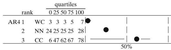
Fig. 15 Analysis #2 PF results for the SOFTLAB projects where NN_{pf} > WC_{pf}
