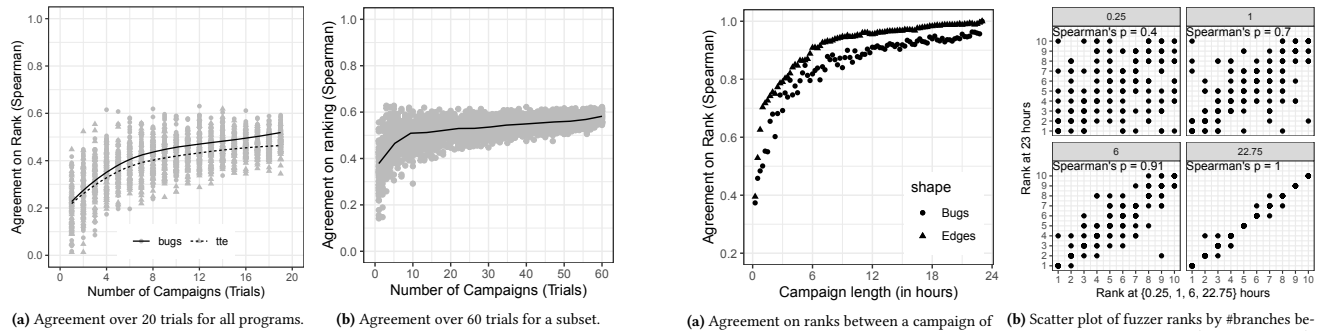
Figure 11: Agreement within coverage- or bug-based benchmarking as campaign length increases.
