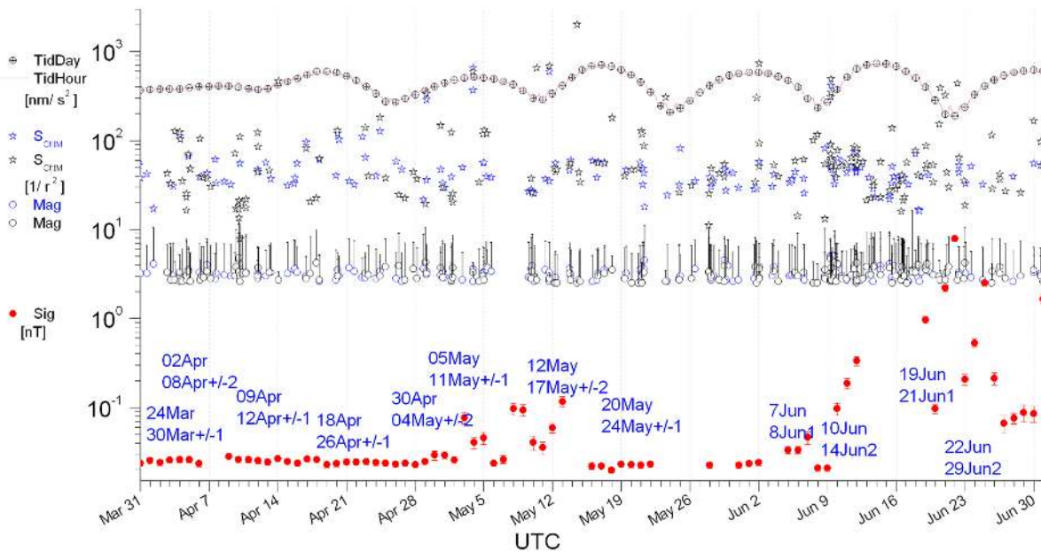
Fig. 9. The reliability of the time window prediction for incoming earthquake, April–June 2003, Sofia region.
