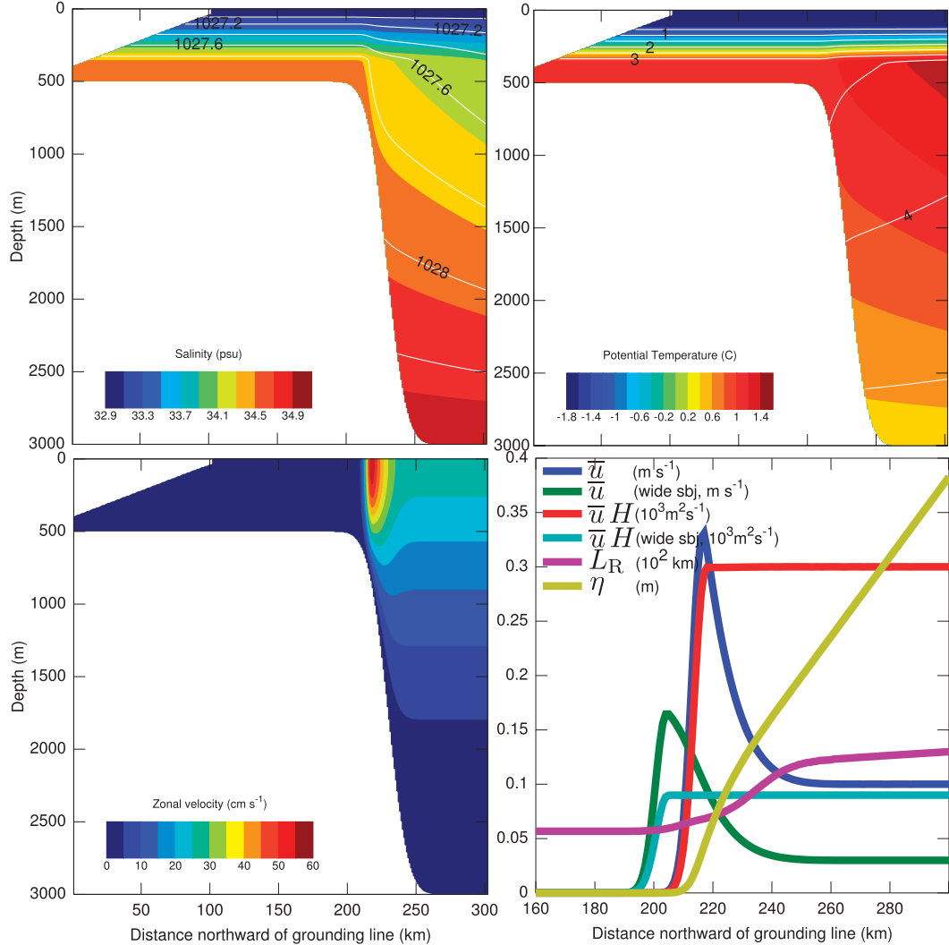
FIG. 2. Initial and boundary conditions used in runs 1, 5, 6, 7, and 11. (top left) Salinity S and neutral density \gamma (contour lines), (top right) potential temperature T and temperature T above in situ freezing point (contour lines), (bottom left) zonal velocity (positive eastward/out of the page), and (bottom right) cross-shelf variation of various parameters are shown. See text for definition of symbols.
