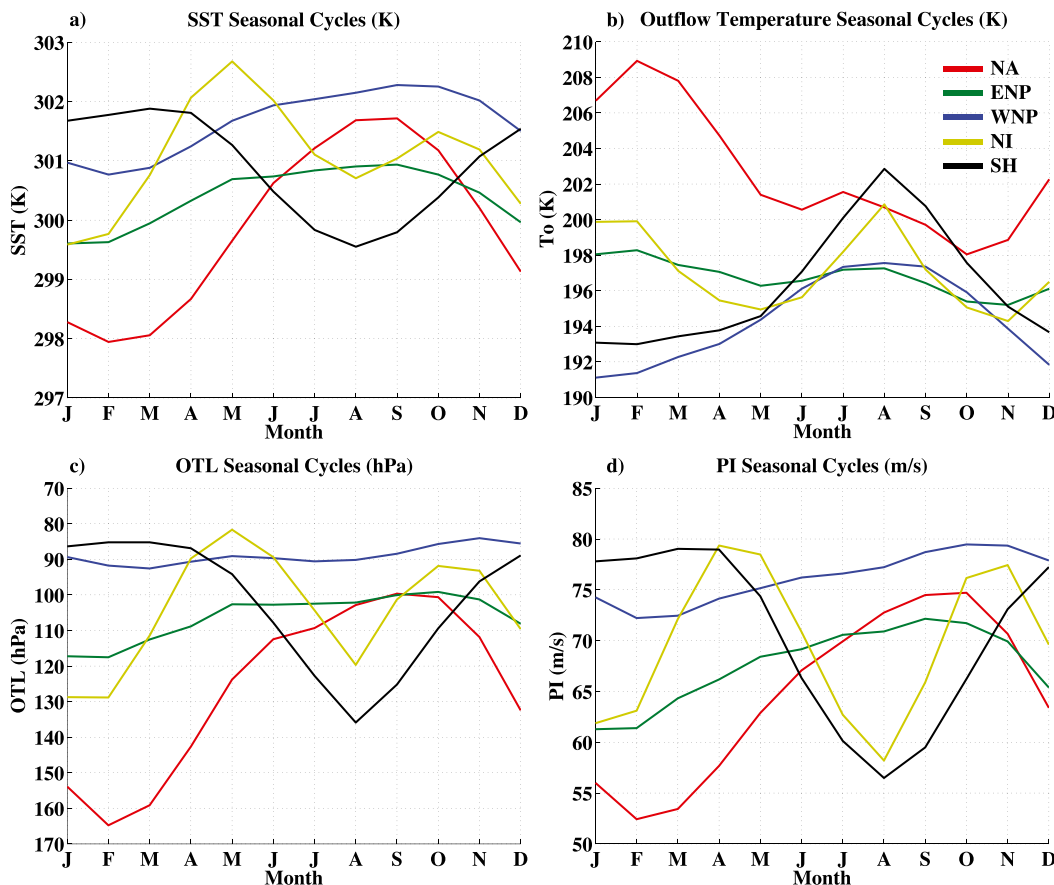
FIG. 1. Seasonal cycles of (a) SST, (b) TC outflow temperature, (c) OTL, and (d) TC PI using MERRA-2 data averaged over 1980–2013 and the TC development regions. The main development regions are NA (red), ENP (green), WNP (blue), NI (yellow), and SH (black), as defined in Table 1.
