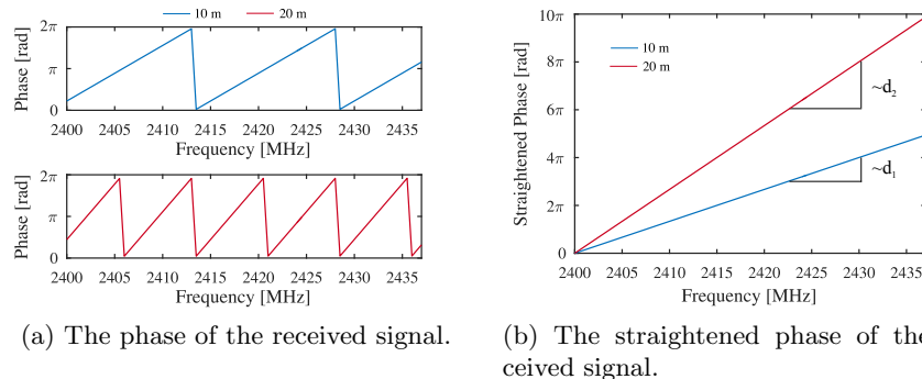
Fig. 2: Phase versus frequency if the prover is 10 and 20 m away from the verifier.
