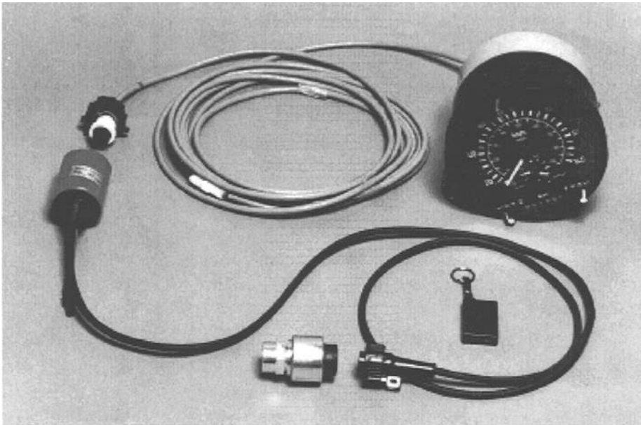
Fig. 1. A tachograph with an interruptor controlled using a radio key fob.
