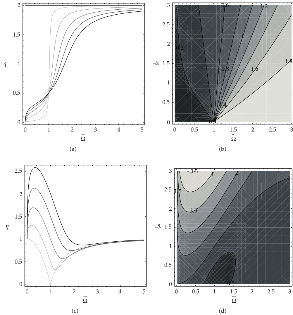
Figure 4: Plots of q and \eta for p = 0.50 . (a) q(\tilde{\Omega}, \xi) versus \tilde{\Omega} for \xi = 0.1, 0.5, 1, 1.5, and 2 (going from light to dark). The asymptotic behavior is similar to the case when p = 0.25 . (b) Map of q(\tilde{\Omega}, \xi) where lower values are represented by darker colors. When \tilde{\Omega} = 1 , q = 0.50 for any value of \xi . (c) \eta(\tilde{\Omega}, \xi) versus \tilde{\Omega} for \xi = 0.1, 0.5, 1, 1.5, and 2 (going from light to dark). (d) Map of \eta(\tilde{\Omega}, \xi) .
