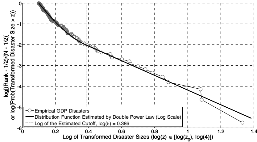
Log GDP Disaster Sizes vs. \log[(\text{Rank} - 1/2)/(N - 1/2)] and Estimated Distribution Function (Log Scale) (Double Power Law, z_0 = 1.105 )
