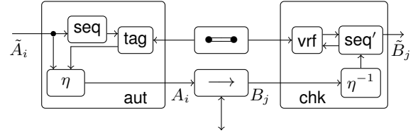
Figure 4: The authentication protocol (aut, chk) is based on the MAC scheme (tag, vrf). The systems seq and seq' handle sequence numbers; \eta and \eta^{-1} convert the message-tag pairs for the message space of \longrightarrow .
