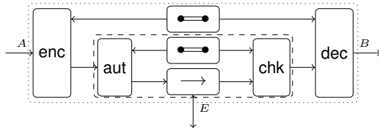
(a) Encrypt-then-Authenticate, the structure is described as \text{enc}^A \text{dec}^B (\text{aut}^A \text{chk}^B (\rightarrow \parallel \bullet \bullet) \parallel \bullet \bullet) below.
