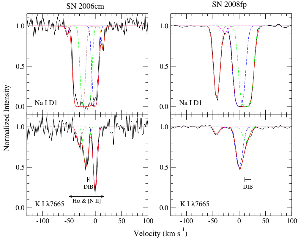
Figure 4. Host Na I D1 and K I \lambda 7665 absorption in SNe 2006cm and 2008fp. The observations correspond to the black line. The best-fitting VPFIT model is shown as the red line, with the individual Voigt profile components plotted as dashed lines. Zero velocity has been arbitrarily set to correspond to the strongest component of the K I \lambda 7665 profile. The velocities of the 5780 Å DIB in each SN are shown as \pm 1\sigma error bars, and were derived assuming a Gaussian profile of 2.1 Å FWHM and a rest wavelength of 5780.55 Å (Taurisg et al. 2000). The FWHM velocity range covered by the H \alpha and [N II] emission in the extracted spectrum of SN 2006cm is also indicated.
