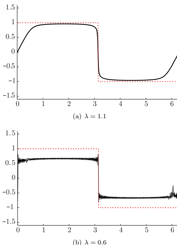
FIGURE 2. Solutions of system (7.3) with N = 256 , T = 0.5 , and \epsilon_N = 0 . The piecewise constant initial datum is u_0(x) = \text{sgn}(\pi - x) .
