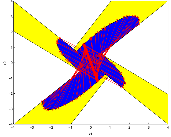
Fig. 1. State-feedback: State trajectories - red; \mathcal{X}_T - blue polyhedra; \mathcal{X}_U - yellow and blue polyhedra.
