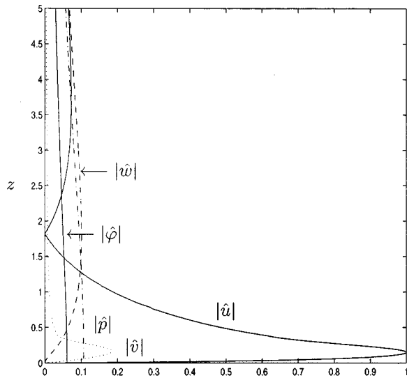
FIG. 6. Magnitude of all nonzero eigenfunctions normalized by the maximum in \hat{u} for R=50\,000 on the upper branch of the marginal curve for a wall-normal imposed magnetic field, for an insulating boundary and for k_y = \pm 0.01 : — |\hat{u}| ; - - - |\hat{w}| ; - · - |\hat{p}| ; · · · |\hat{v}| ; - · · |\hat{\phi}| .
