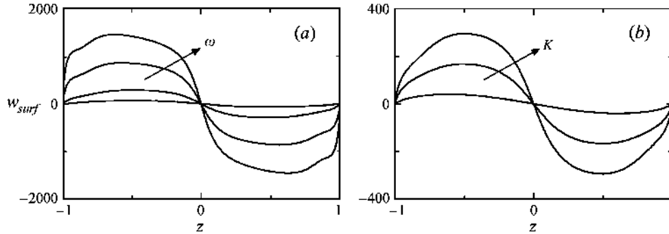
FIGURE 6. Free-surface velocity for A = 1 , \delta = 1 . (a) K = 1000 and 8\omega/3 = 0.5, 2, 4 and 5 . (b) 8\omega/3 = 2 and K = 100, 500 and 1000 .
