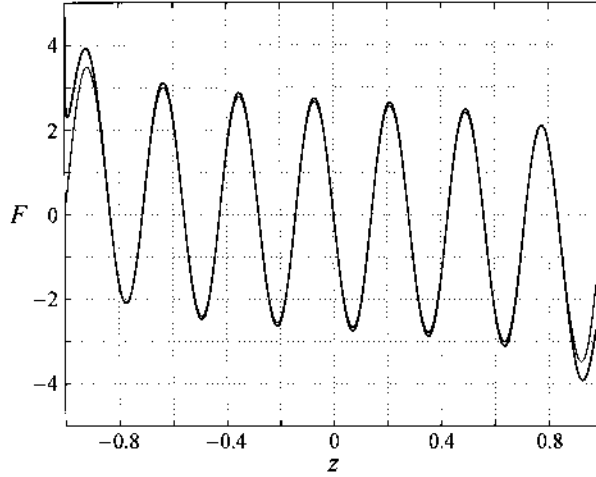
FIGURE 4. The function F for A = 1 , \Omega = 104 and \beta_+ = \beta_- = 1 : as given by (4.2) (thick line) and as calculated in Nicolás et al. (1997) (thin line).
