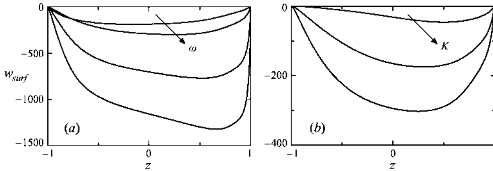
FIGURE 8. Free-surface velocity for A = 1 , \delta = 0 . (a) K = 1000 and 8\omega/3 = 0.5, 2, 4 and 5 . (b) 8\omega/3 = 2 and K = 100, 500 and 1000 .
