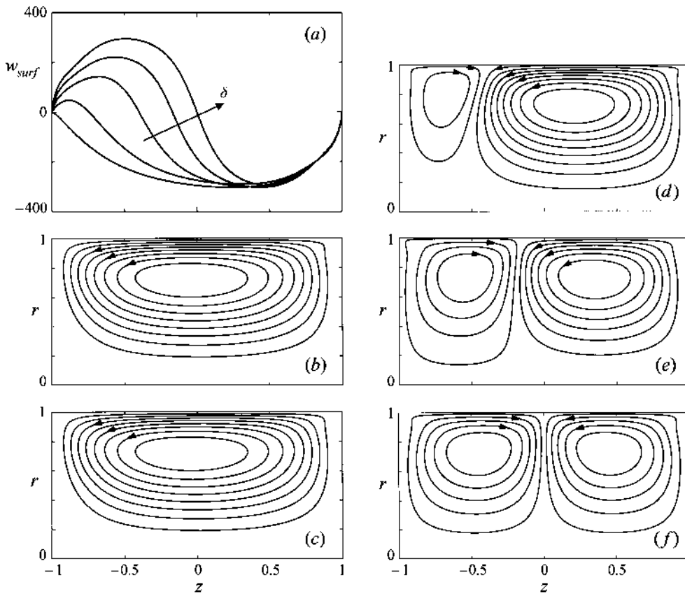
FIGURE 9. (a) Free-surface velocity for the values of the parameters in (b)–(f). (b)–(f) Streamlines for A = 1 , K = 1000 , 8\omega/3 = 2 and \delta = 0, 0.25, 0.5, 0.75 and 1 respectively.
