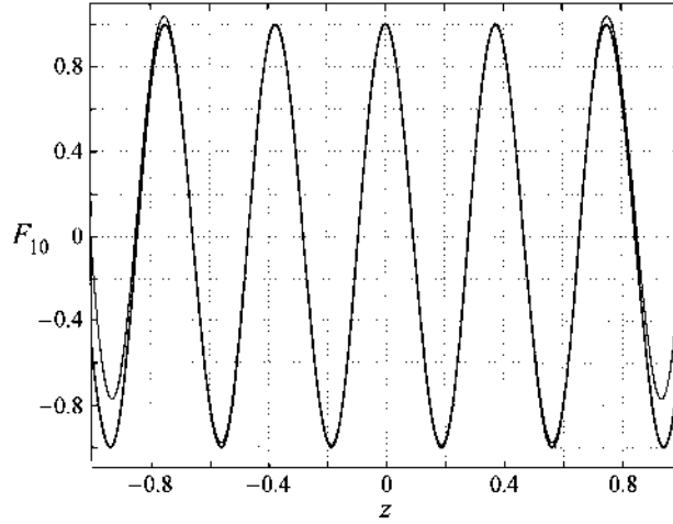
FIGURE 3. The tenth eigenfunction F_{10} for A = 1 : as given by (4.7) (thick line) and as calculated in Sanz (1985) (thin line).
