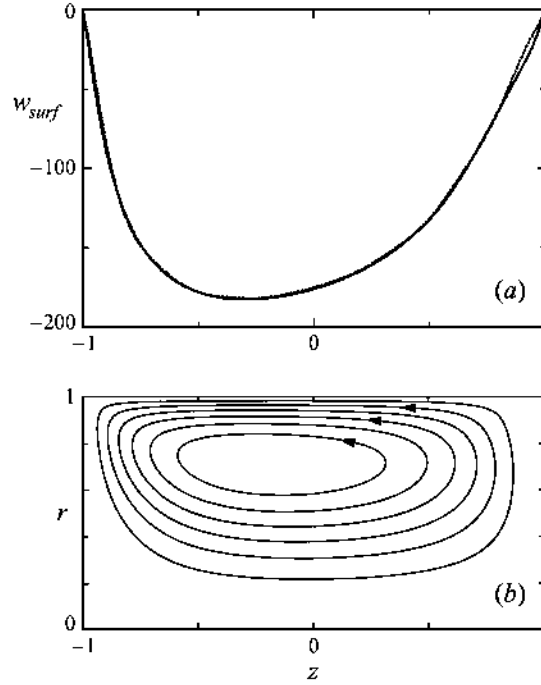
FIGURE 5. Comparison of high-frequency (solid lines) and low-frequency (dotted lines) models: (a) free-surface velocity, (b) streamlines.
