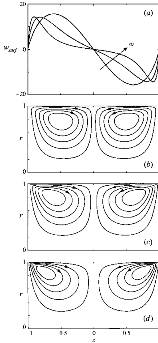
FIGURE 7. (a) Free-surface velocity for the values of the parameters in (b)–(d). (b)–(d) Streamlines for A = 1 , \delta = 1 and (\omega, K) = (0.5, 195.9) , (5, 3.415) and (10, 0.04540) respectively.
