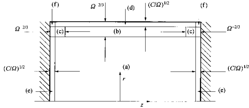
FIGURE 1. Sketch of the six distinguished regions in the liquid bridge.
