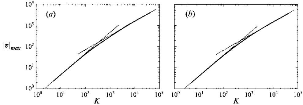
FIGURE 10. Maximum velocity modulus as a function of K , for A = 1 and 8\omega/3 = 2 . (a) Vibration of one disk ( z = +A ): \delta = 0.0180 . (b) Vibration of both disks in phase or counterphase: \delta = 1 . Dotted lines correspond to asymptotes of slope 1 and 2/3 .
