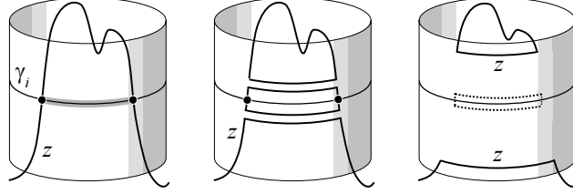
FIGURE 5. A cycle z such that z \cdot [\gamma_i] = 0 can be moved out of \mathcal{C}_i^{max} .
