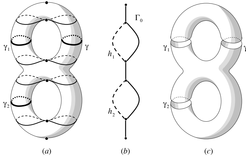
FIGURE 4. Proof of Theorem 2.1.
