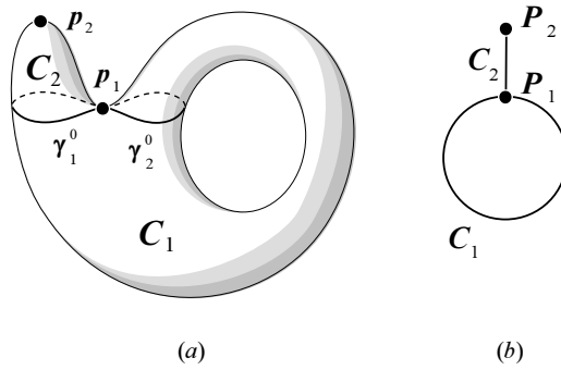
FIGURE 2. (a) The leaf \gamma_2^0 adjoins only one component, while \gamma_1^0 connects two components. (b) The corresponding foliation graph has a loop.
