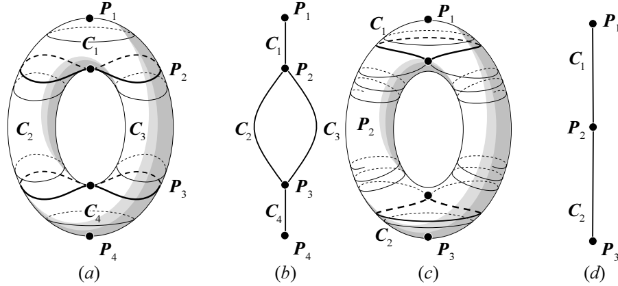
FIGURE 3. (a), (c) Examples of the decomposition. (b) The vertices of \Gamma can include singularities, non-compact compactifiable leaves and (d) whole minimal components.
