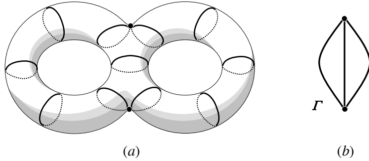
FIGURE 6. (a) The foliation from Example 4.1 and (b) its foliation graph.
