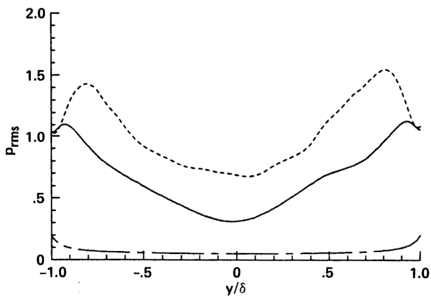
Figure 1. Root-mean-square fluctuation for each pressure according to equation (3): ———, rapid; - - - - , slow; - · - · , Stokes.
