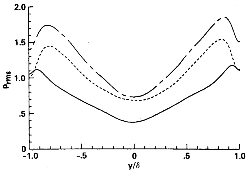
Figure 2. Root-mean-square fluctuation for each pressure according to equation (2): ———, rapid; - - - - , slow; - · - · , total.
