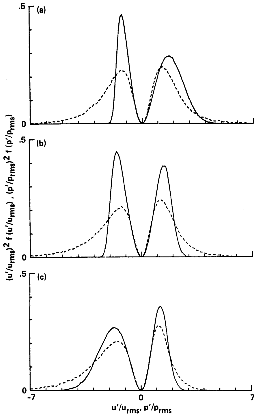
Figure 6. Fractional contributions to the mean-square fluctuation: —, u' ; ----, p' . The abscissa is normalized by the corresponding local rms fluctuations and the ordinate is normalized such that the area under the curve is equal to one: (a) y^+ = 0 for p and y^+ = 5 for u ; (b) y^+ = 12 ; (c) y^+ = 100 .
