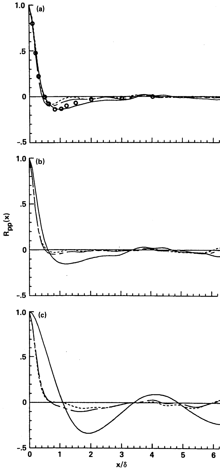
Figure 10. Two-point correlations of the rapid (—), slow (----), and total (-·-·-) pressure in the streamwise direction: (a) y^+ = 0 ; (b) y^+ = 50 ; (c) y^+ = 180 . The symbols represent the results obtained by Lee (1989) using the rapid distortion theory.
