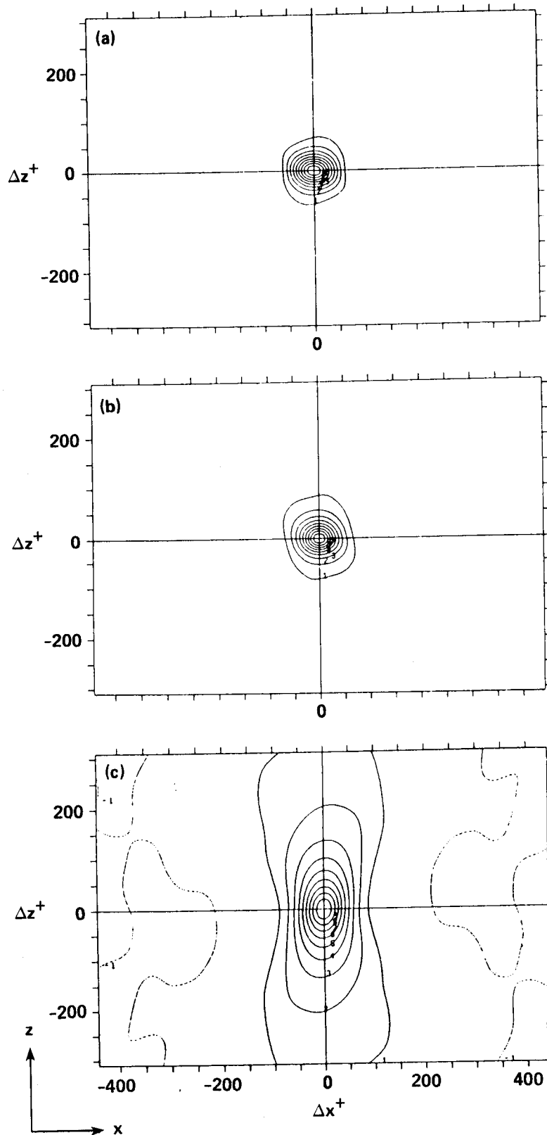
Fig. 11 Contours of constant two-point correlations of the total pressure fluctuations, R_{pp}(r_x, r_z) : (a) y^+ = 0 ; (b) y^+ = 50 ; (c) y^+ = 180 . The contour level '1' corresponds to 0.1 and higher levels are incremented by 0.1, and the tick marks in the axes represent 50 wall units.
