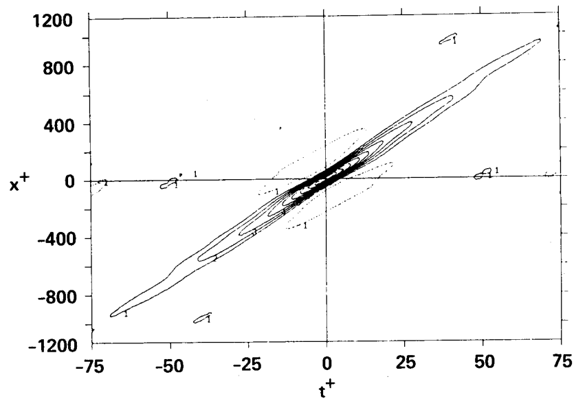
Fig. 16 Space-time correlation of the wall-pressure fluctuations, R_{pp}(r_x, r_t) .
