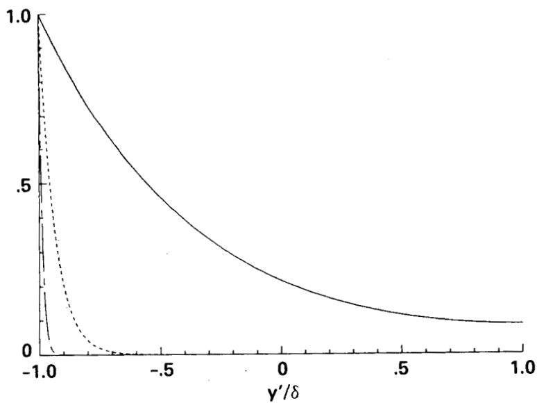
Fig. 17 Green's function for three different wave numbers: —, k_x\delta = 2\pi/(\lambda_x/\delta) = 0.5 and k_z\delta = 2\pi/(\lambda_z/\delta) = 1.5 ; ----, k_x\delta = 5 and k_z\delta = 15 ; -·-·, k_x\delta = 25 and k_z\delta = 75 . Each Green's function is normalized such that its maximum value is equal to one.
