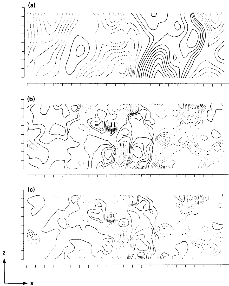
Fig. 22 Contours of constant (a) rapid, (b) slow, and (c) total pressure at the centerline. The mean flow direction is from left to right, and the tick marks denote 50 wall units.
