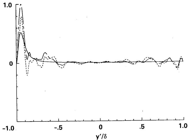
Fig. 19 Contribution to the mean-square wall-pressure fluctuation from across the channel: —, rapid pressure; ----, slow pressure; -·-·, total pressure. The ordinate is normalized such that the maximum value is equal to one.
