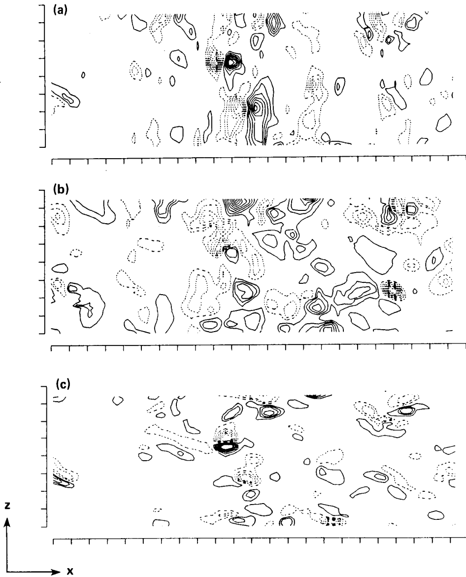
Fig. 24 Contours of constant (a) \partial p/\partial x , (b) \partial p/\partial y and (c) \partial p/\partial z at the centerline. The mean flow direction is from left to right, and the tick marks denote 50 wall units.
