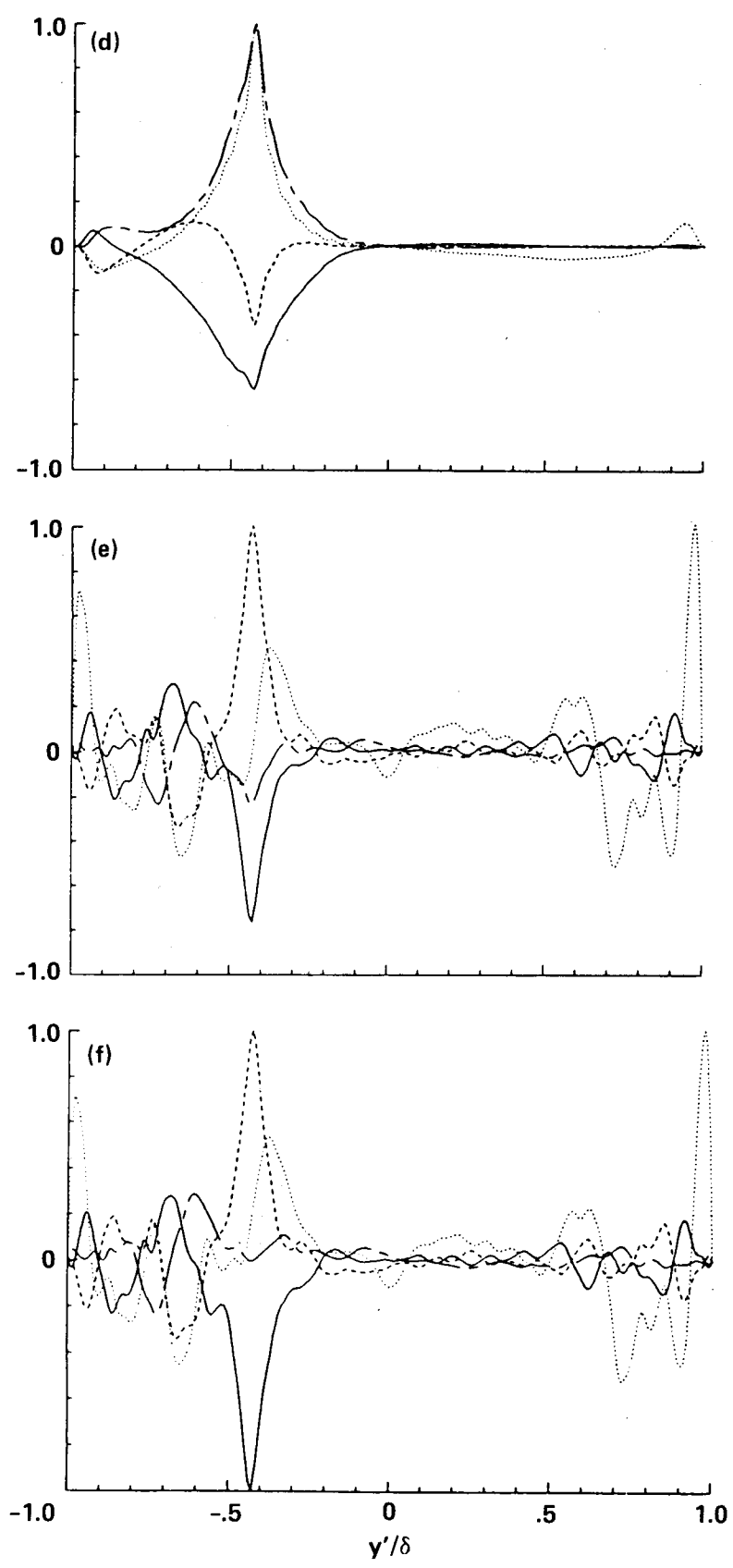
Fig. 20 - continued (d) rapid, (e) slow, and (f) total pressure-strain at y^+ \approx 100 .
