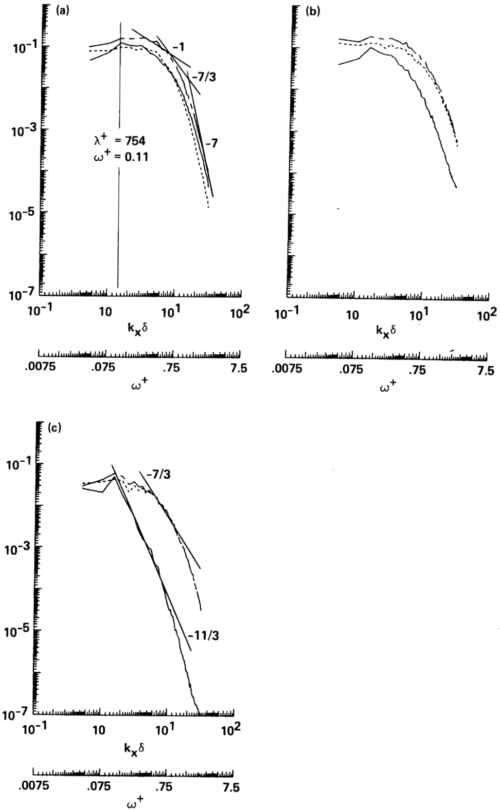
Fig. 9 Power spectra of the rapid (—), slow (---), and total (— · —) pressure in the streamwise direction: (a) y^+ = 0 ; (b) y^+ = 50 ; (c) y^+ = 180 .
