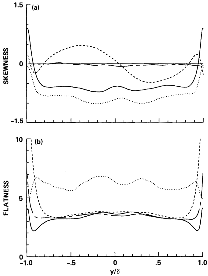
Figure 7. (a) Skewness and (b) flatness factors of the velocity and pressure fluctuations: —, u ; ---, v ; - · -, w ; ·····, p .
