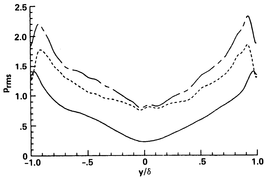
Figure 3. Root-mean-square fluctuation for Re_\tau = 400 : —, rapid; ----, slow; - · - ·, total.
