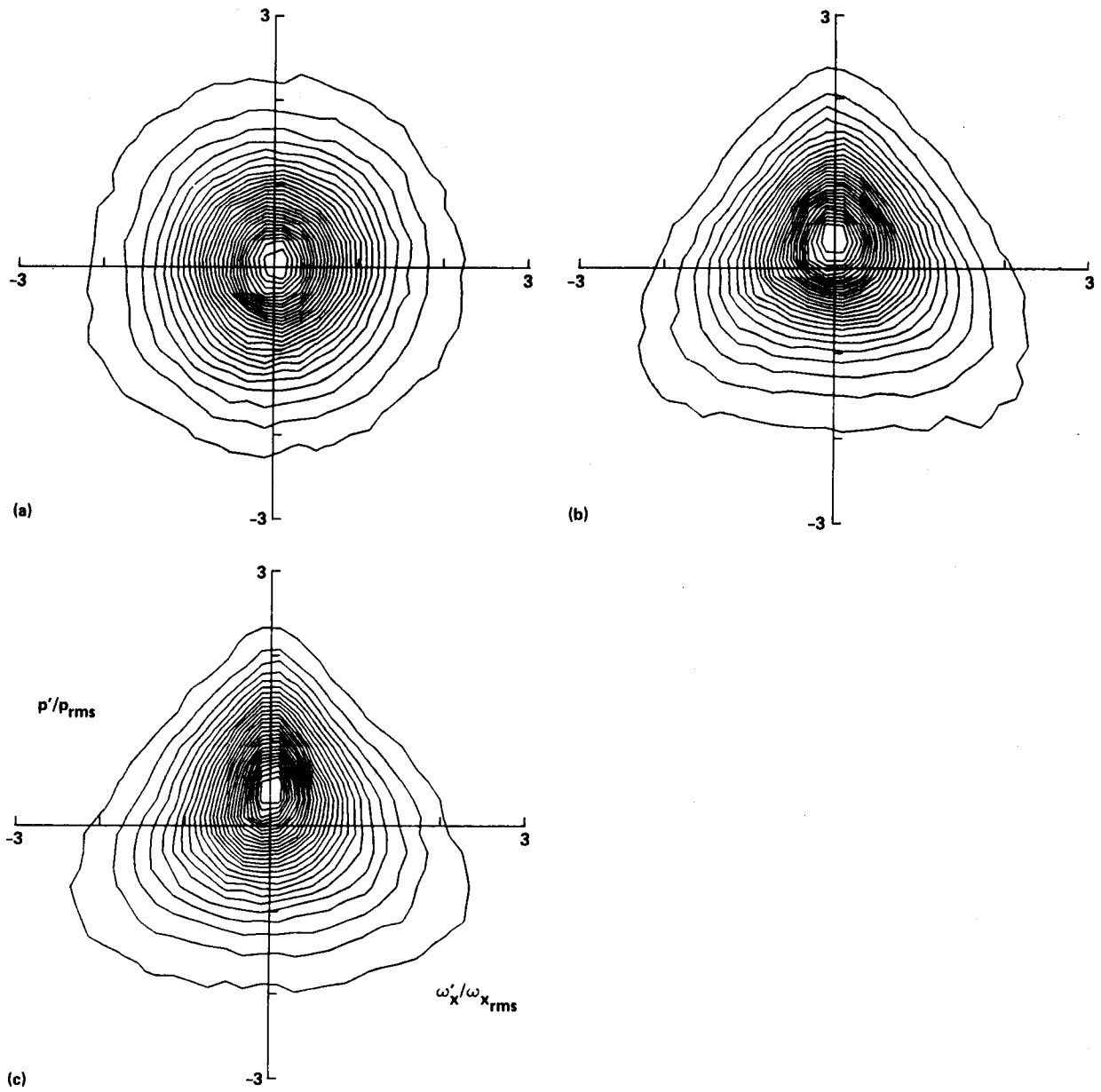
Figure 8. Joint probability density distribution between p' and w'_x : (a) y^+ = 0 ; (b) y^+ = 30 ; (c) y^+ = 100 . The axes are normalized by the corresponding rms fluctuations.
