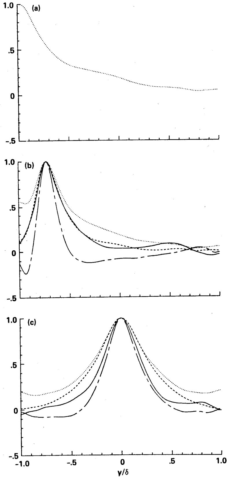
Fig. 15 Two-point correlations in the normal direction, R_{ii}(y) : —, R_{uu} ; ---, R_{vv} ; - - - , R_{ww} ; ..... , R_{pp} . (a) y^+ = 0 ; (b) y^+ = 50 ; (c) y^+ = 180 .
