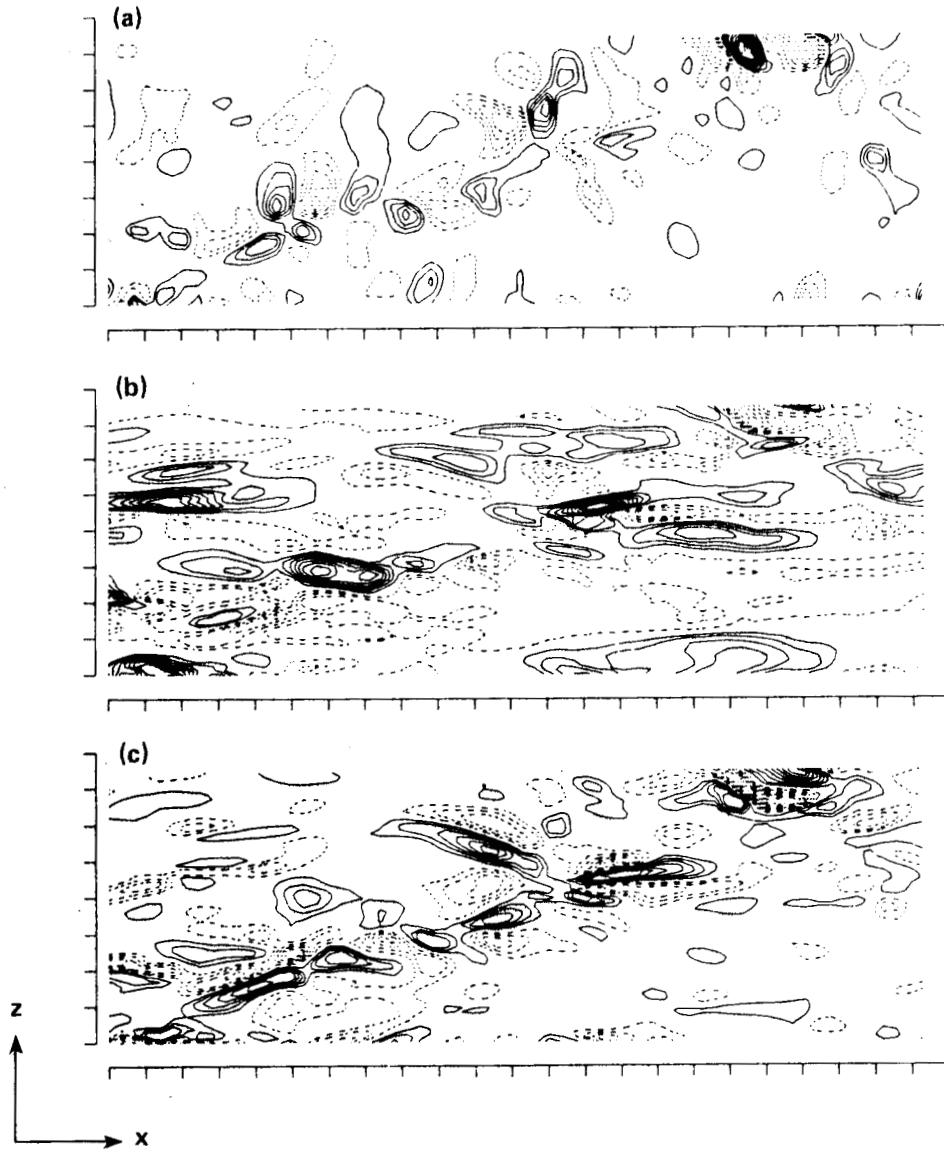
Fig. 23 Contours of constant (a) \partial p/\partial x , (b) \partial p/\partial y , and (c) \partial p/\partial z at the wall. The mean flow direction is from left to right, and the tick marks denote 50 wall units.
