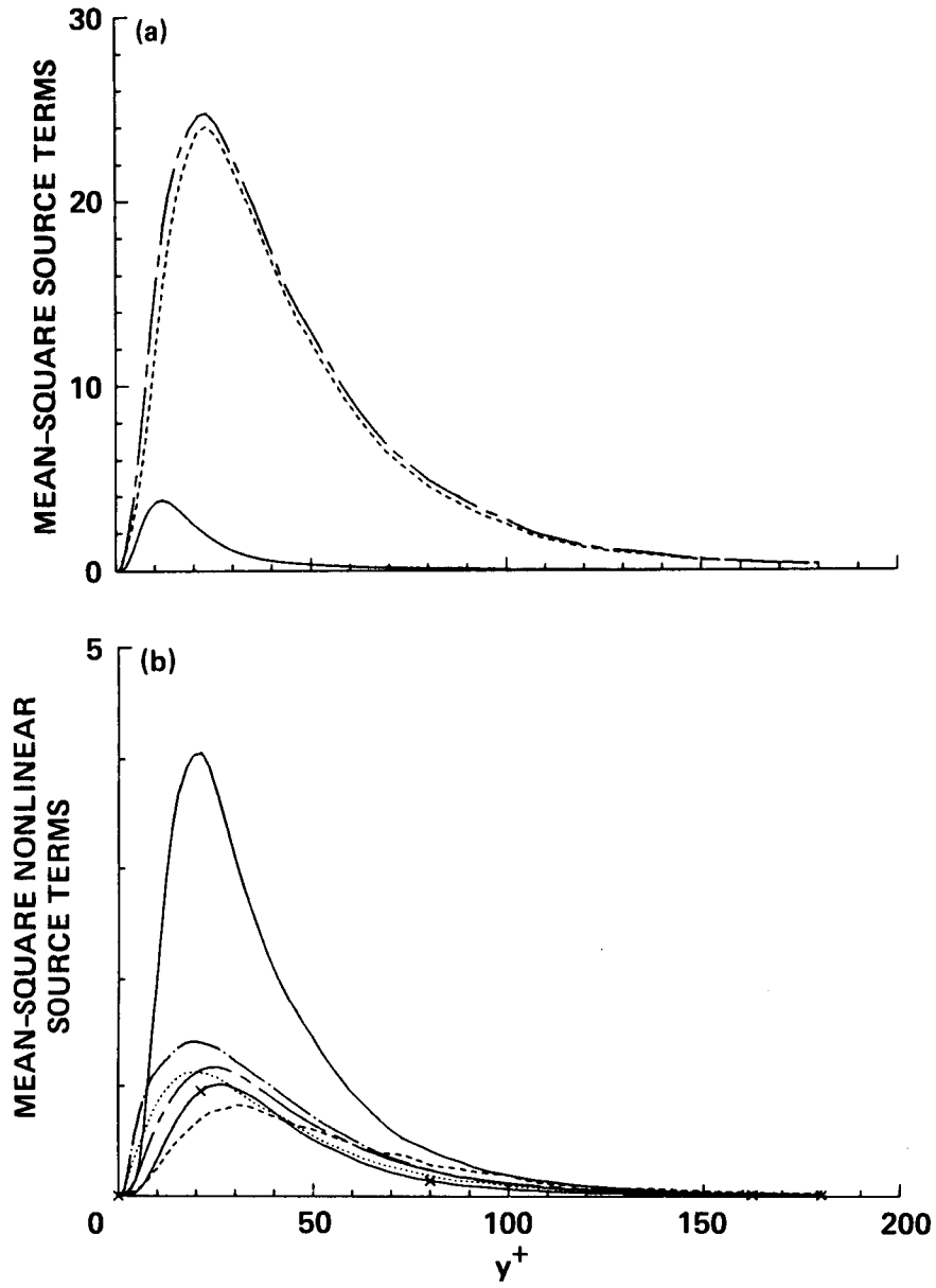
Figure 4. Profiles of the mean-square source terms. (a) ———, linear; - - - - , nonlinear; - · - · , total. (b) Profiles of the mean-square nonlinear terms: ———, (\partial u' / \partial x)^2 ; - - - - , (\partial u' / \partial y)(\partial v' / \partial x) ; - · - · , (\partial u' / \partial z)(\partial w' / \partial x) ; ······ , (\partial v' / \partial y)^2 ; ———, (\partial v' / \partial z)(\partial w' / \partial y) ; - - - - , (\partial w' / \partial z)^2 .
