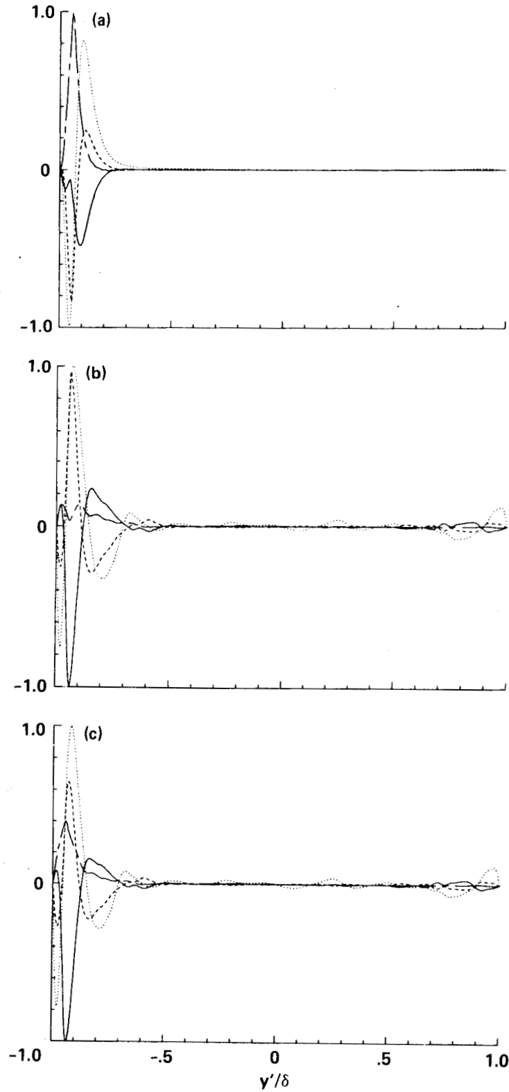
Fig. 20 Contributions to the pressure-strain correlations: —, \overline{2p(\partial u/\partial x)} ; ----, \overline{2p(\partial v/\partial y)} ; ---, \overline{2p(\partial w/\partial z)} ; ·····, \overline{p(\partial u/\partial y + \partial v/\partial x)} . The ordinate is normalized such that the maximum value of the four terms is equal to one. (a) rapid, (b) slow, and (c) total pressure-strain at y^+ \approx 10 ;
