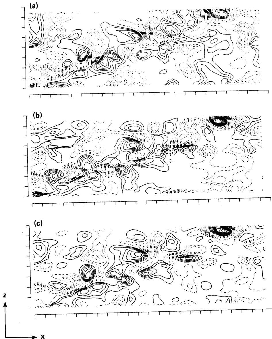
Fig. 21 Contours of constant (a) rapid, (b) slow, and (c) total pressure at the wall. The mean flow direction is from left to right, and the tick marks denote 50 wall units.
