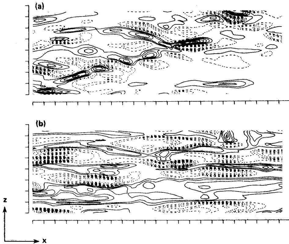
Fig. 25 Contours of constant (a) streamwise and (b) spanwise vorticity at the wall.
