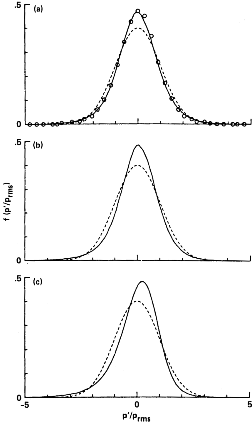
Figure 5. Probability density distribution of the total pressure-fluctuations: — , computation; ---- , Gaussian distribution; o , Schewe (1983). The abscissa is normalized by the local rms pressure fluctuations and the ordinate is normalized such that the area under the curve is equal to one: (a) y^+ = 0 ; (b) y^+ = 12 ; (c) y^+ = 100 .
