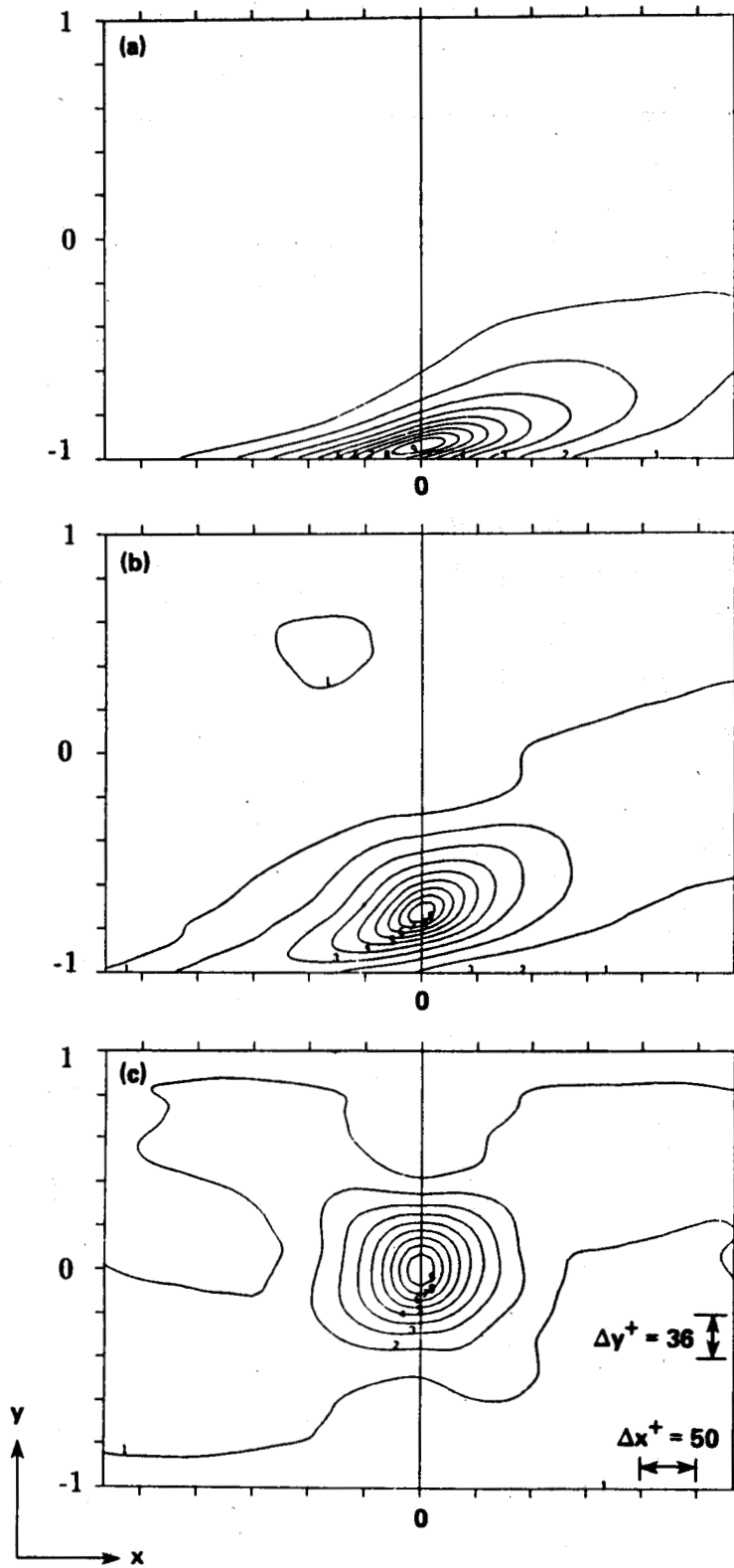
Figure 14. Contours of constant two-point correlations of the streamwise velocity fluctuations, R_{uu}(\Delta x, y, y') : (a) y'^+ = 10 ; (b) y'^+ = 50 ; (c) y'^+ = 180 . Note that \Delta y/\delta = 0.2 corresponds to \Delta y^+ = 36 , and the y -coordinate is stretched by a factor of about two.
