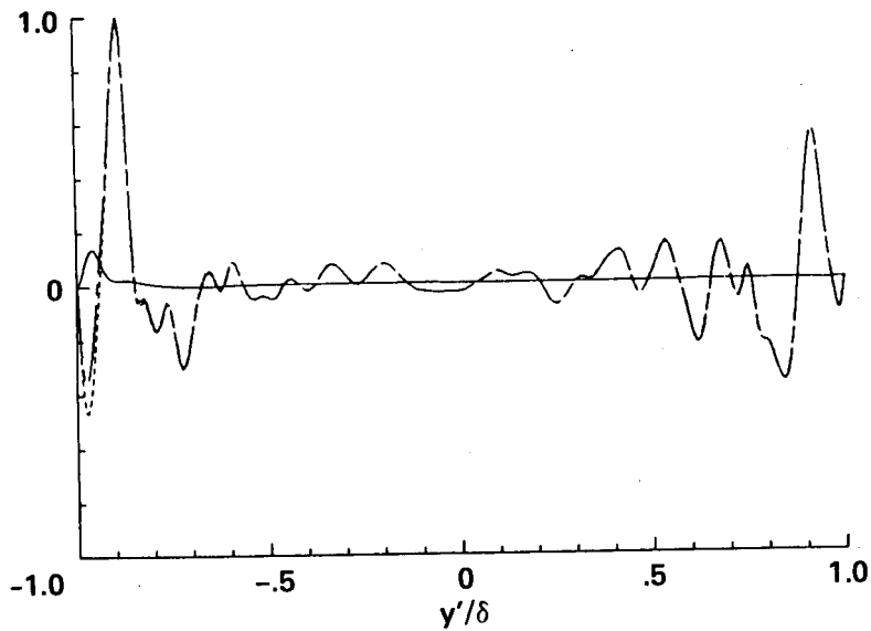
Fig. 18 Contribution to instantaneous wall pressure, p(x = 0, y = -1, z = 0) , from across the channel: —, rapid pressure; ----, slow pressure; -·-·, total pressure. The ordinate is normalized such that the maximum value is equal to one.
