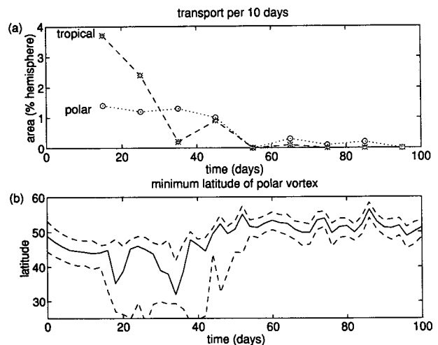
FIG. 23. As in Fig. 22 except for the adiabatic calculation shown in Fig. 2.
