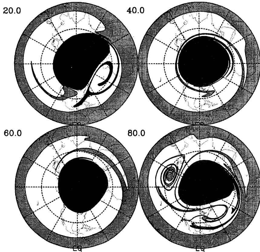
FIG. 18. Results from four 10-day CA calculations, using the winds from the shallow-water calculation shown in Fig. 8, initialized at day (a) 10, (b) 30, (c) 50, and (d) 70. Each calculation was initialized with the PV = 0.25 \times 10^{-8} and 1.125 \times 10^{-8} \text{ m}^{-1} \text{ s}^{-1} contours. Map projection is the same as in Fig. 17.
