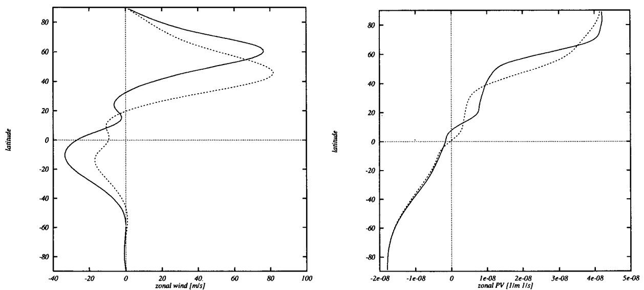
FIG. 16. Zonally averaged (a) wind and (b) potential vorticity profiles at t = 100 days for experiments identical to the one in Fig. 14 except with different forcing amplitudes: H_B = 1000 m (dashed line) and H_B = 2000 m (solid line). Note how increasing the amplitude shifts the regions of steep PV gradients poleward.
