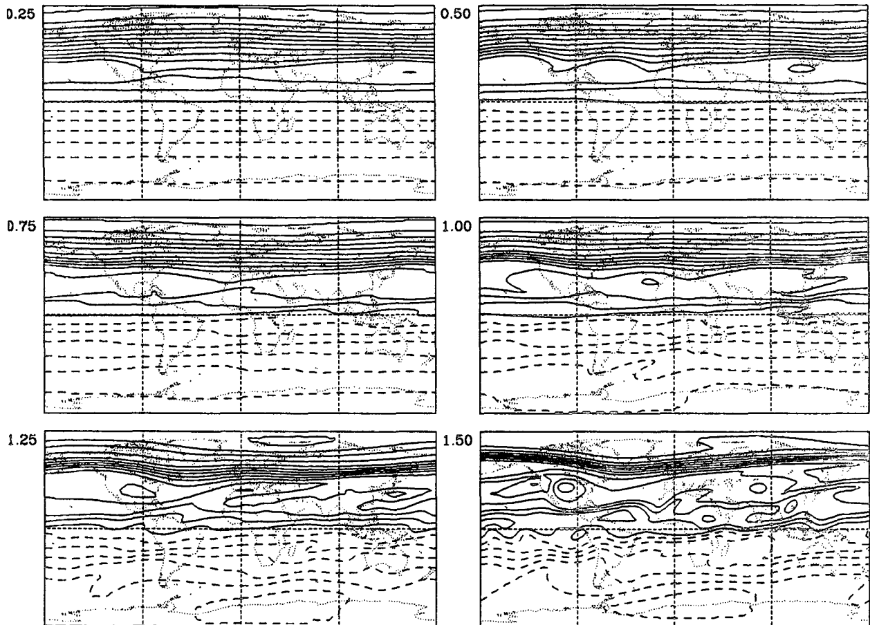
FIG. 5. The PV field at t = 50 days for six calculations with parameters identical to the one in Fig. 2, except for the forcing amplitude H_B , whose values in km is given next to each frame (the last frame is from Fig. 2). The contour intervals are as in Fig. 2.
