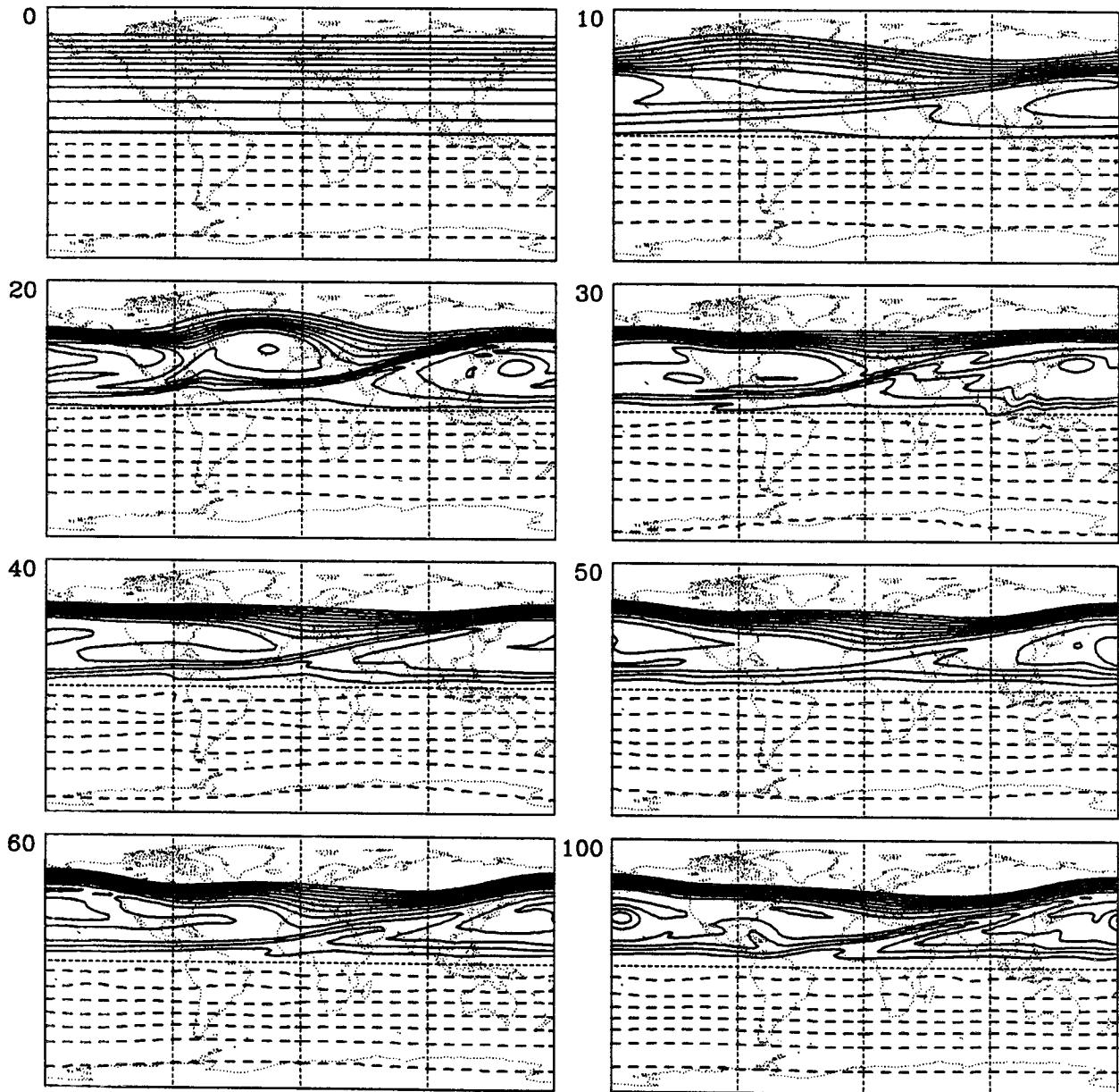
FIG. 8. The response of a polar vortex to topographic forcing in the presence of thermal relaxation; \tau_E = 10 days and h_E as given in Fig. 7. See caption to Fig. 2.
