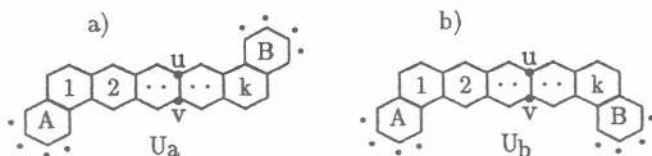
Figure 1. Two unbranched catacondensed benzenoid systems used to illustrate the concept of subgraphs R_x , R_y and R_{xy} ; for details see text.
