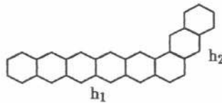
Figure 2. An unbranched catacondensed benzenoid system with two segments.
