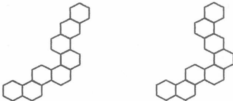
Figure 3. Two unbranched catacondensed benzenoid systems with 8 hexagons, having equal Szeged indices ( S_z = 7969 ); this is the same value as the Wiener index of [12]helicene.
